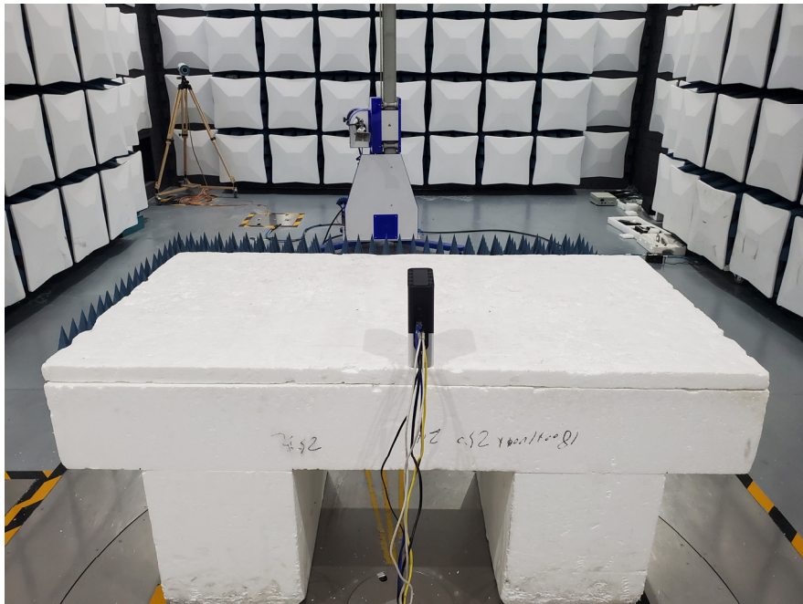
Radiated Disturbances Side View (18-30GHz)
