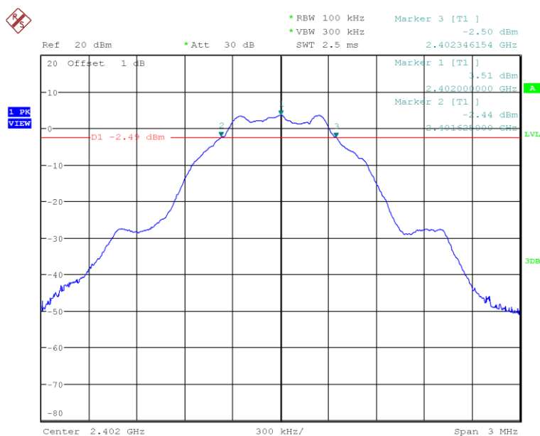
Fig.7 6dB Bandwidth: Ch0
