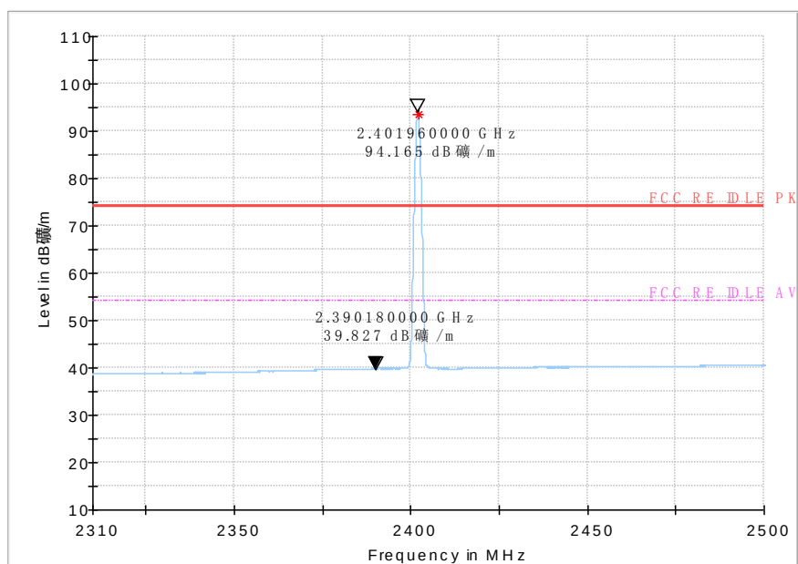
Fig.29 Bandedge:ch0
