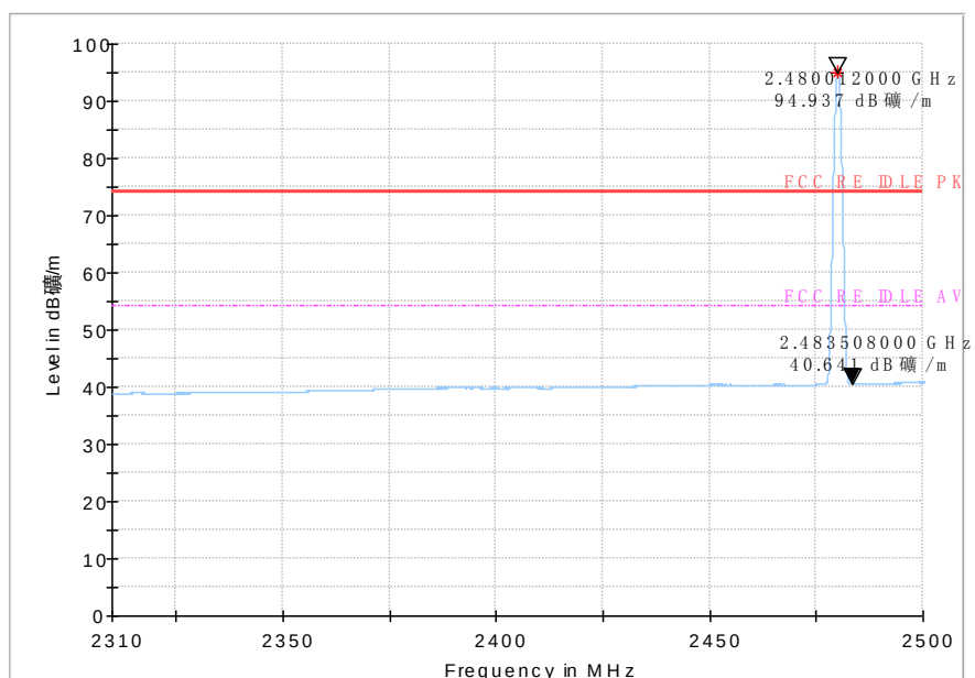
Fig.25 Bandedge: Ch39
