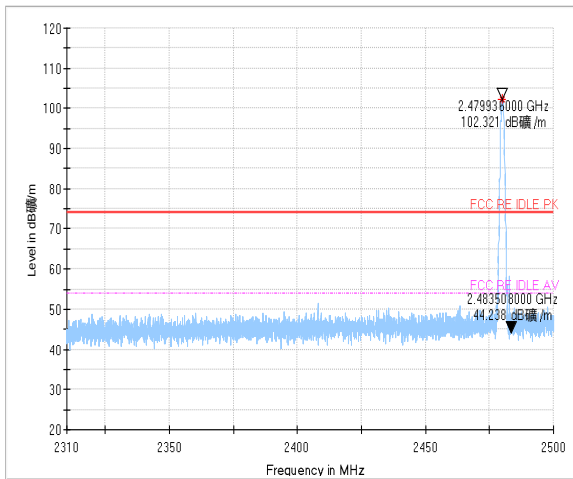
Bandedge (High): GFSK, high channel
