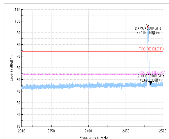
Bandedge: Ch39
