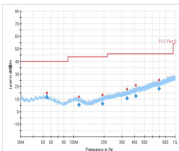
Radiated emission: Ch0, 30MHz~1GHz
