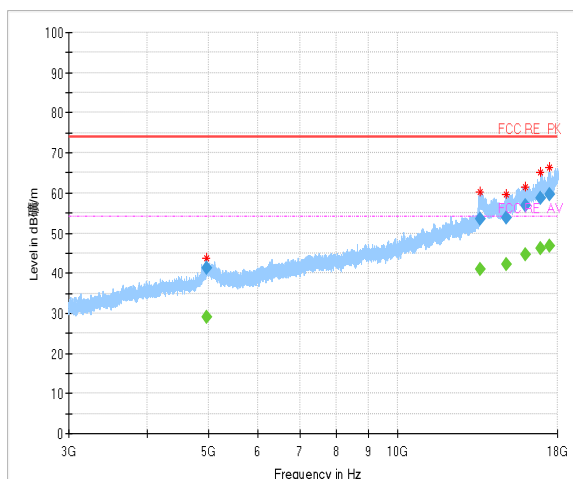
Radiated emission: Ch39, 3GHz~18GHz
