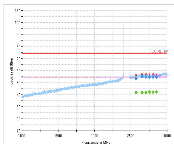
Radiated emission: Ch0, 1GHz~3GHz
