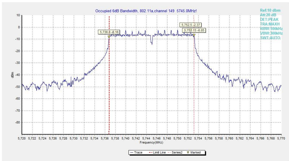
Fig. 19 Occupied 6dB Bandwidth (802.11a, 5745MHz)
