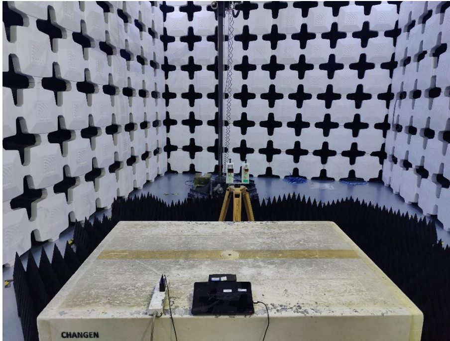
3. Radiated Emissions (Part 15B Video Player, 18GHz-26.5GHz)
