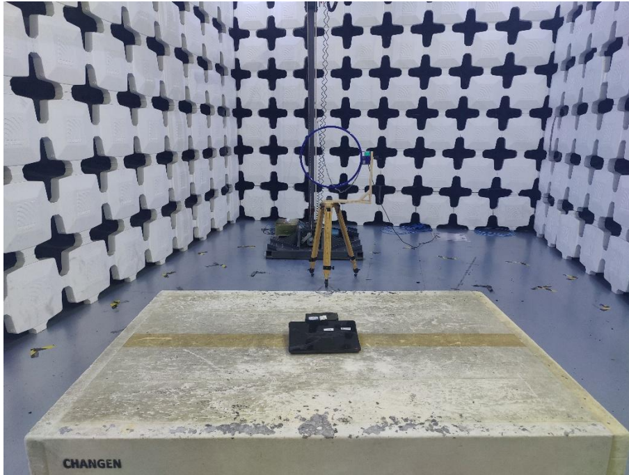
5. Radiated Emissions (Part 15C NFC, 9kHz-30MHz)
