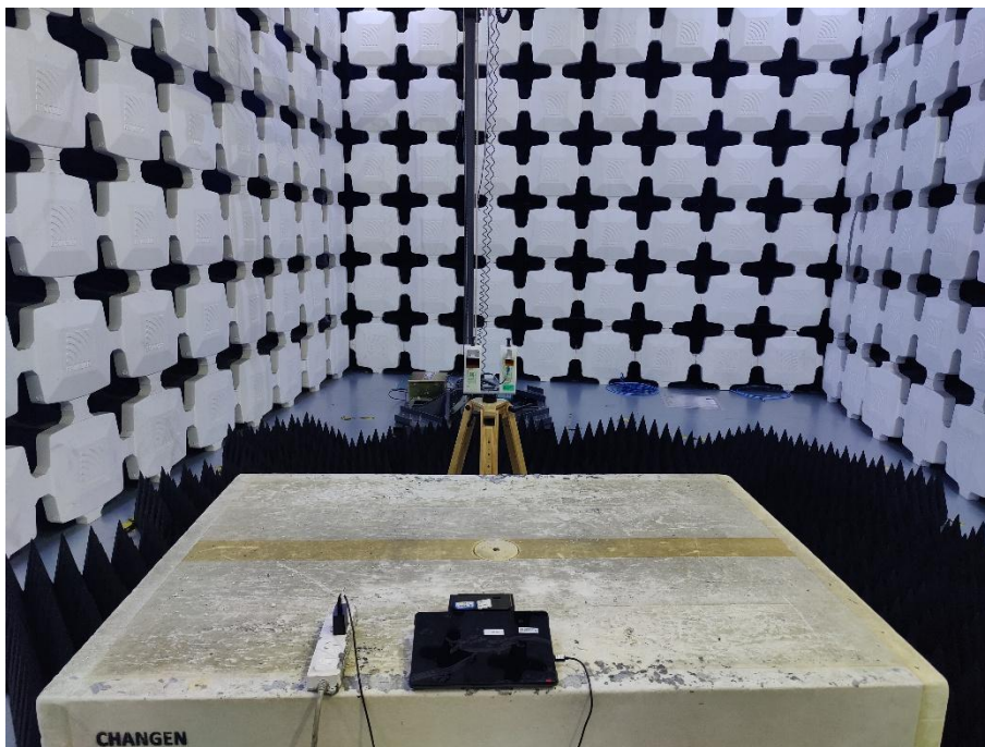
4. Radiated Emissions (Part 15B Video Player, 26.5GHz-40GHz)
