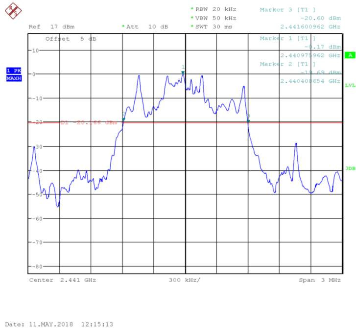
Fig.80 20dB Bandwidth: 8DPSK, Ch39
