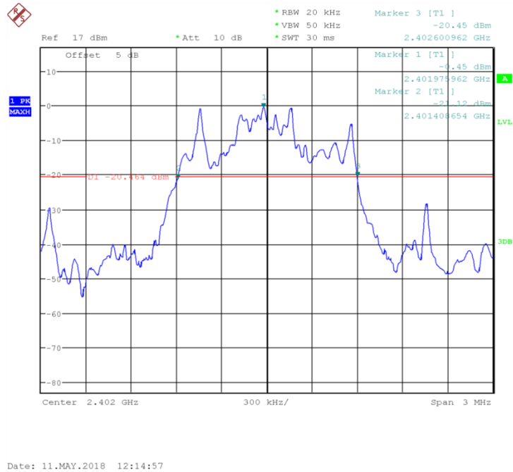
Fig.79 20dB Bandwidth: 8DPSK, Ch0
