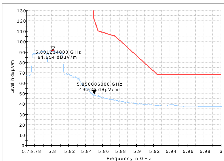
Fig. 78 Band Edges (802.11n-HT40, 5795MHz)
