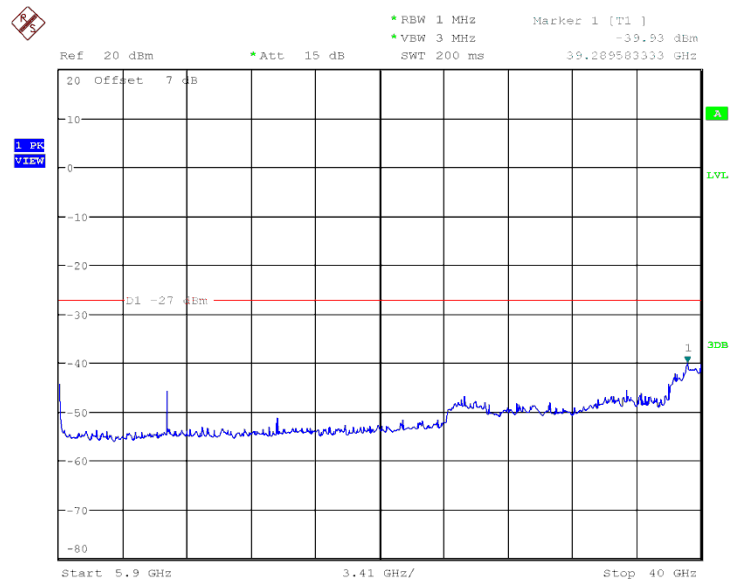
Fig. 26 Conducted Spurious Emission (802.11n-HT20, Ch165, 5.9 GHz-40 GHz)
