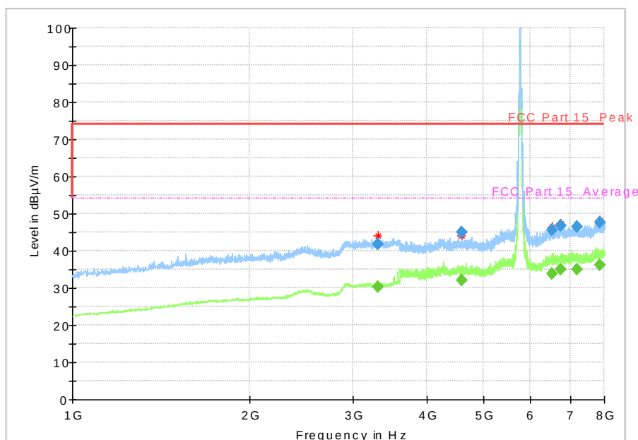
Fig. 64 Radiated Spurious Emission (802.11n-HT40, Ch159, 1 GHz-8 GHz)
