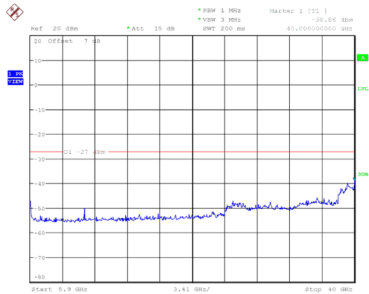
Fig. 32 Conducted Spurious Emission (802.11n-HT40, Ch159, 5.9 GHz-40 GHz)
