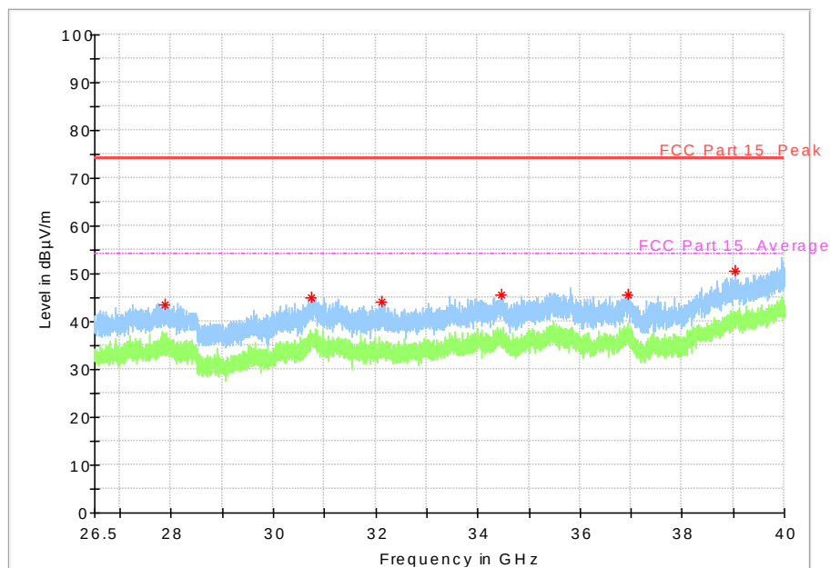
Fig. 72 Radiated emission: 802.11n, (802.11n-HT40, Ch159, 26.5 GHz - 40 GHz)
