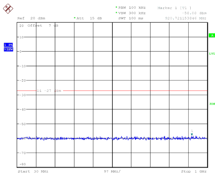
Fig. 21 Conducted Spurious Emission (802.11n-HT20, Ch157, 30 MHz-1 GHz)
