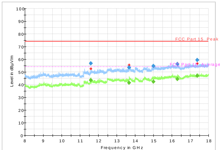
Fig. 70 Radiated Spurious Emission (802.11n-HT40, Ch159, 8 GHz-18 GHz)
