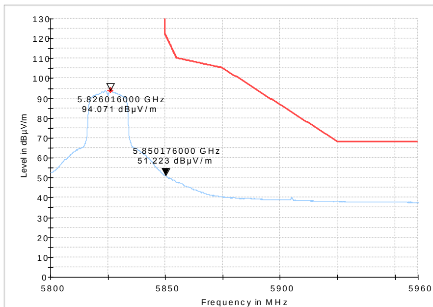
Fig. 74 Band Edges (802.11a, 5825MHz)
