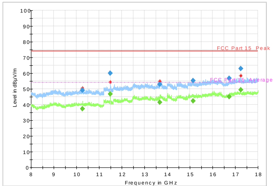
Fig. 35 Radiated Spurious Emission (802.11a, Ch149, 8 GHz-18 GHz)
