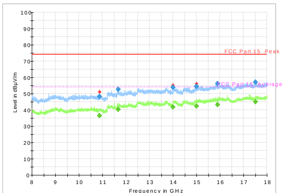
Fig. 65 Radiated Spurious Emission (802.11n-HT40, Ch159, 8 GHz-18 GHz)
