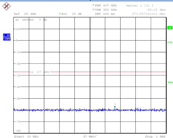
Fig. 12 Conducted Spurious Emission (802.11a, Ch157, 30 MHz-1 GHz)
