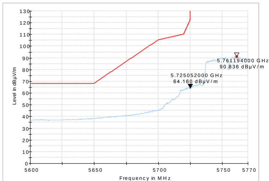
Fig. 77 Band Edges (802.11n-HT40, 5755MHz)
