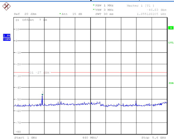
Fig. 16 Conducted Spurious Emission (802.11a, Ch165, 1 GHz -5.6 GHz)
