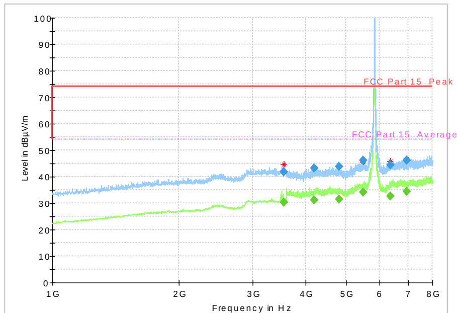
Fig. 44 Radiated Spurious Emission (802.11a, Ch165, 1 GHz-8 GHz)
