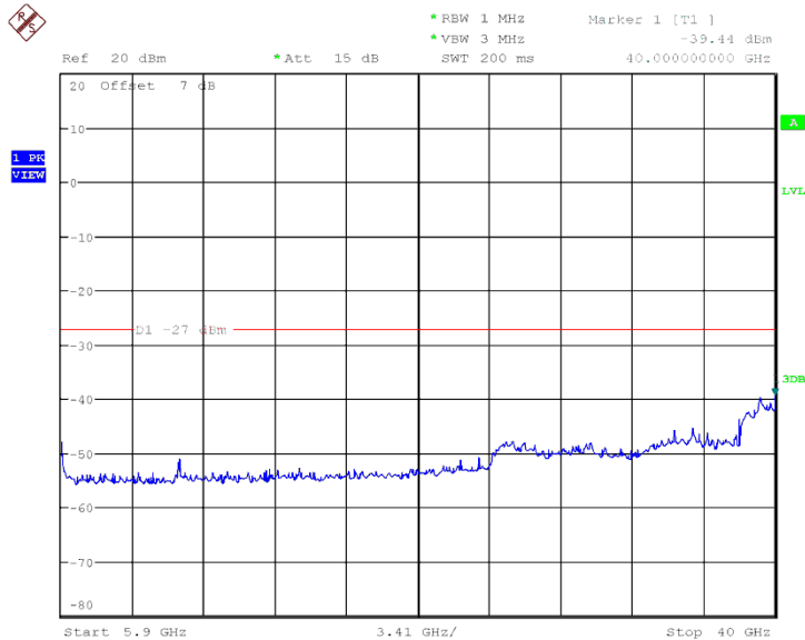
Fig. 29 Conducted Spurious Emission (802.11n-HT40, Ch151, 5.9 GHz-40 GHz)
