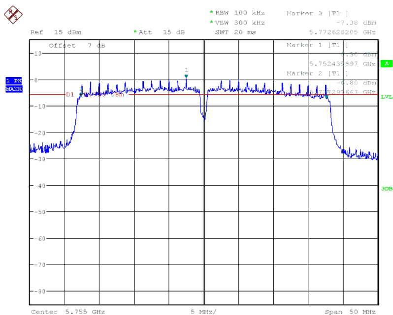
Fig. 7 Occupied 6dB Bandwidth (802.11n-HT40, Ch 151)
