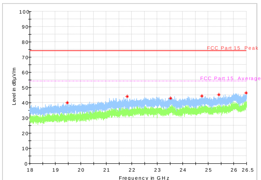
Fig. 66 Radiated Spurious Emission (802.11n-HT40, Ch159, 18 GHz-26.5 GHz)
