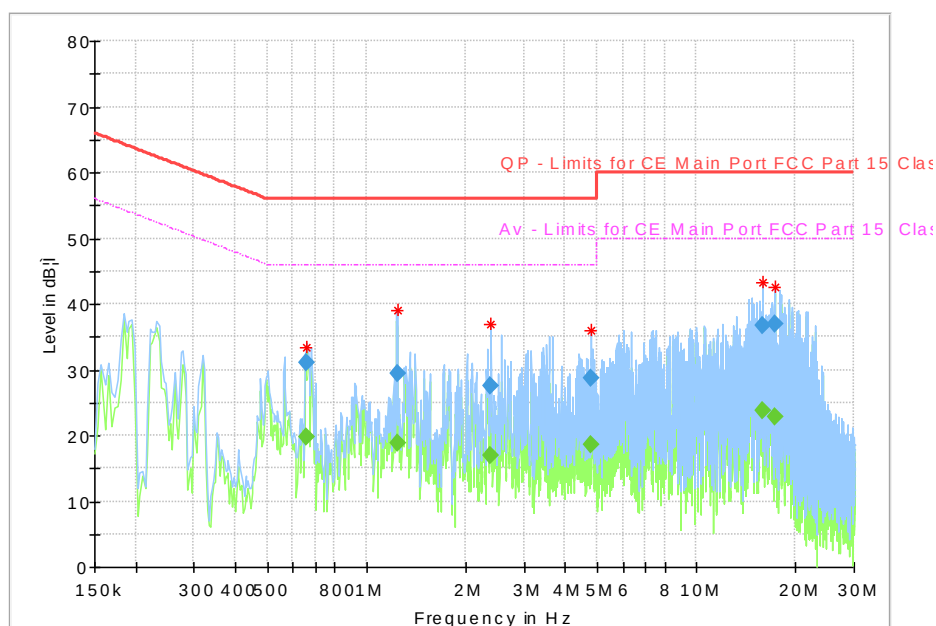
Fig. 79 AC Powerline Conducted Emission-802.11a
