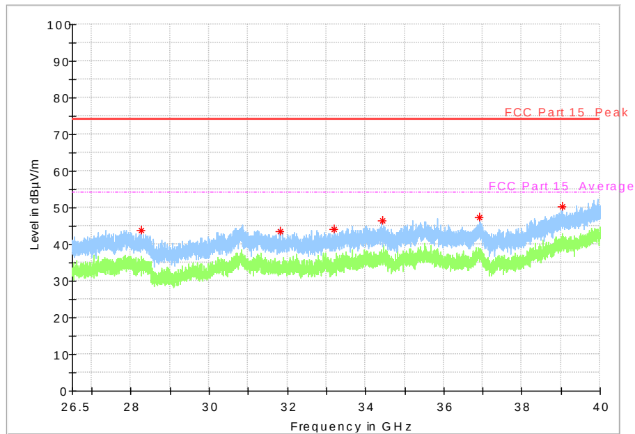
Fig. 57 Radiated emission: 802.11n, (802.11n-HT20, Ch157, 26.5 GHz - 40 GHz)
