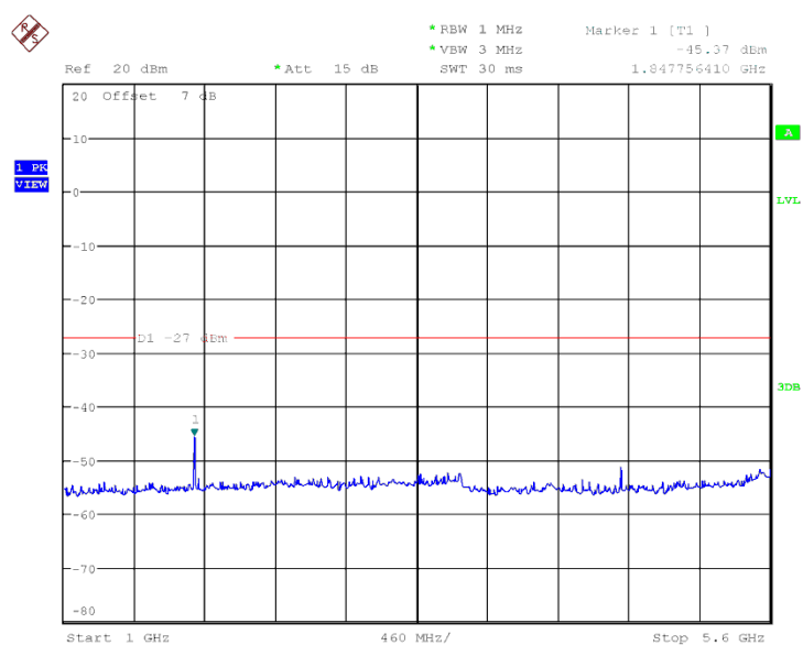
Fig. 13 Conducted Spurious Emission (802.11a, Ch157, 1 GHz-5.6 GHz)
