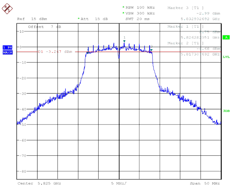
Fig. 3 Occupied 6dB Bandwidth (802.11a, Ch 165)
