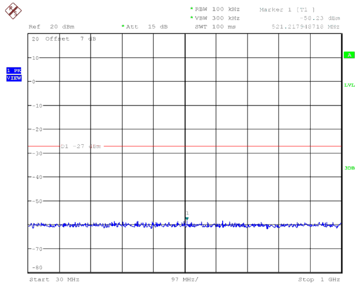
Fig. 30 Conducted Spurious Emission (802.11n-HT40, Ch159, 30 MHz-1 GHz)
