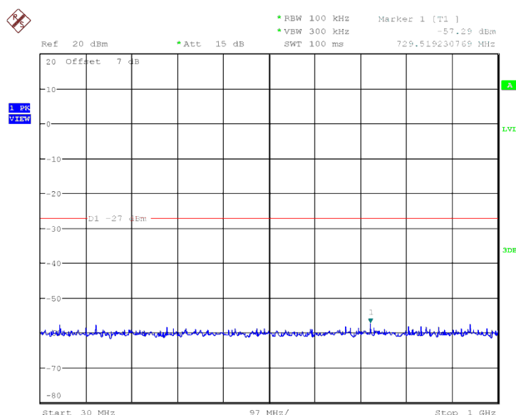
Fig. 9 Conducted Spurious Emission (802.11a, Ch149, 30 MHz-1 GHz)
