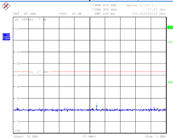
Fig. 18 Conducted Spurious Emission (802.11n-HT20, Ch149, 30 MHz-1 GHz)
