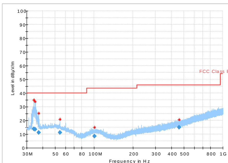
Fig. 63 Radiated Spurious Emission (802.11n-HT40, Ch159, 30 MHz-1 GHz)
