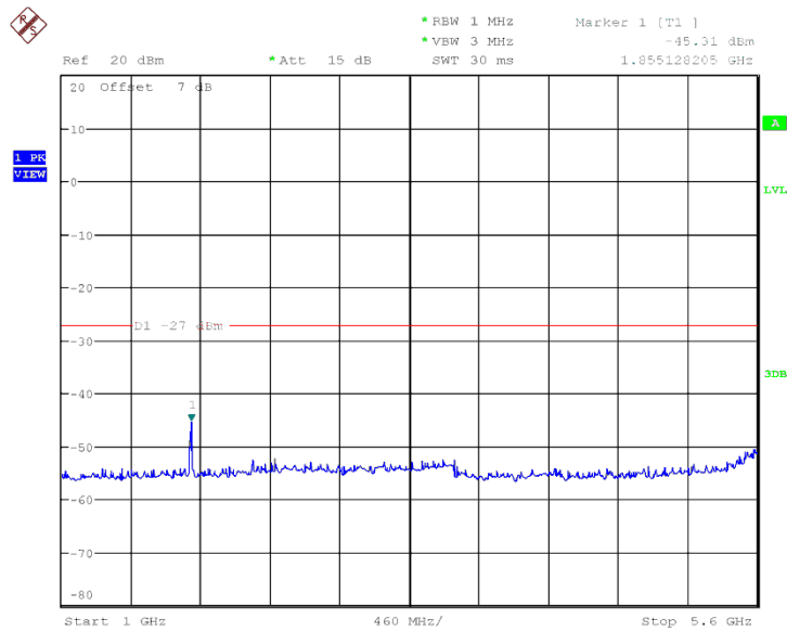
Fig. 28 Conducted Spurious Emission (802.11n-HT40, Ch151, 1 GHz -5.6 GHz)
