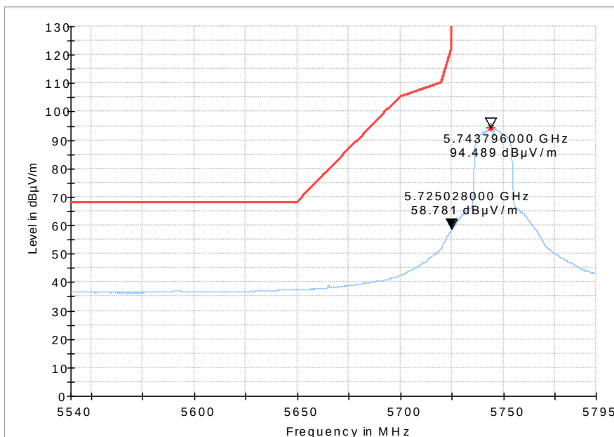
Fig. 73 Band Edges (802.11a, 5745MHz)
