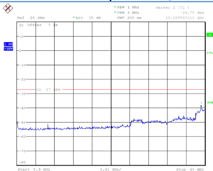
Fig. 20 Conducted Spurious Emission (802.11n-HT20, Ch149, 5.9 GHz-40 GHz)
