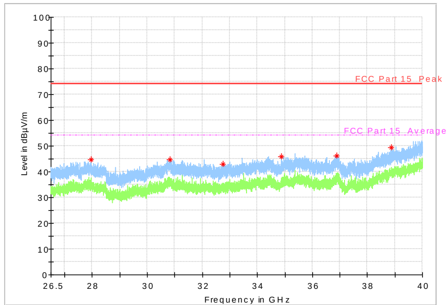
Fig. 47 Radiated emission: 802.11n, (802.11a, Ch165, 26.5 GHz - 40 GHz)
