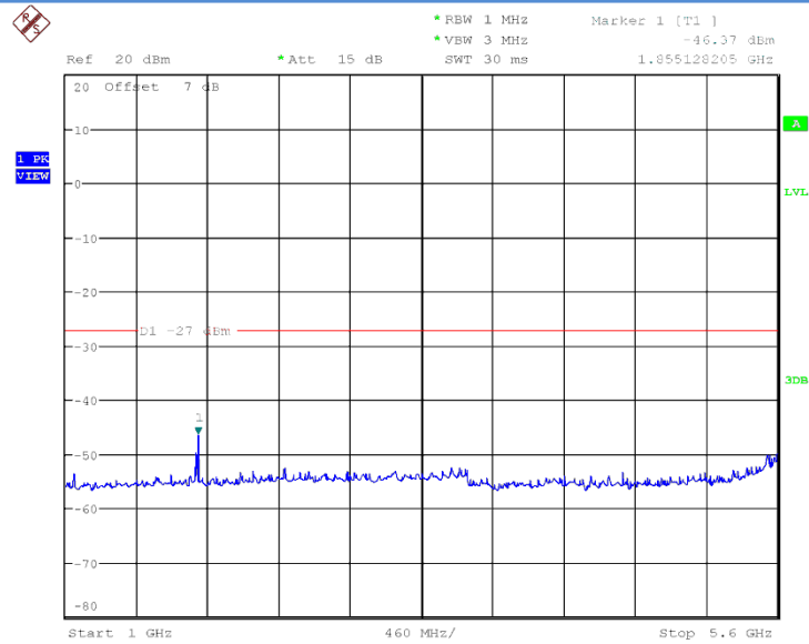
Fig. 10 Conducted Spurious Emission (802.11a, Ch149, 1 GHz -5.6 GHz)
