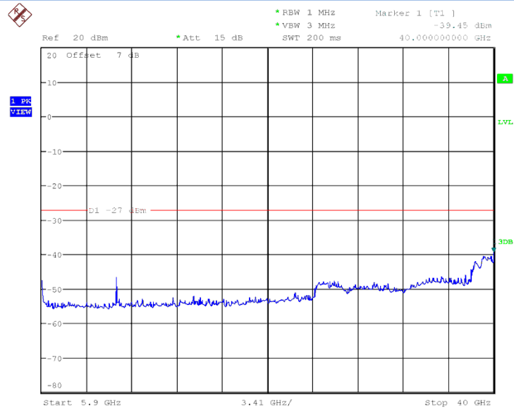
Fig. 14 Conducted Spurious Emission (802.11a, Ch157, 5.9 GHz-40 GHz)
