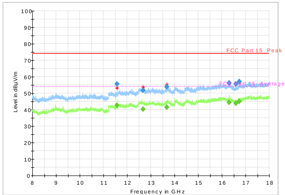
Fig. 55 Radiated Spurious Emission (802.11n-HT20, Ch157, 8 GHz-18 GHz)
