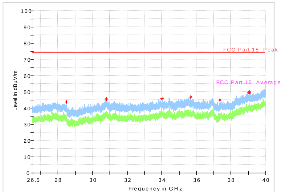
Fig. 67 Radiated emission: 802.11n, (802.11n-HT40, Ch159, 26.5 GHz - 40 GHz)
