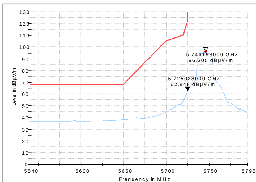
Fig. 75 Band Edges (802.11n-HT20, 5745MHz)
