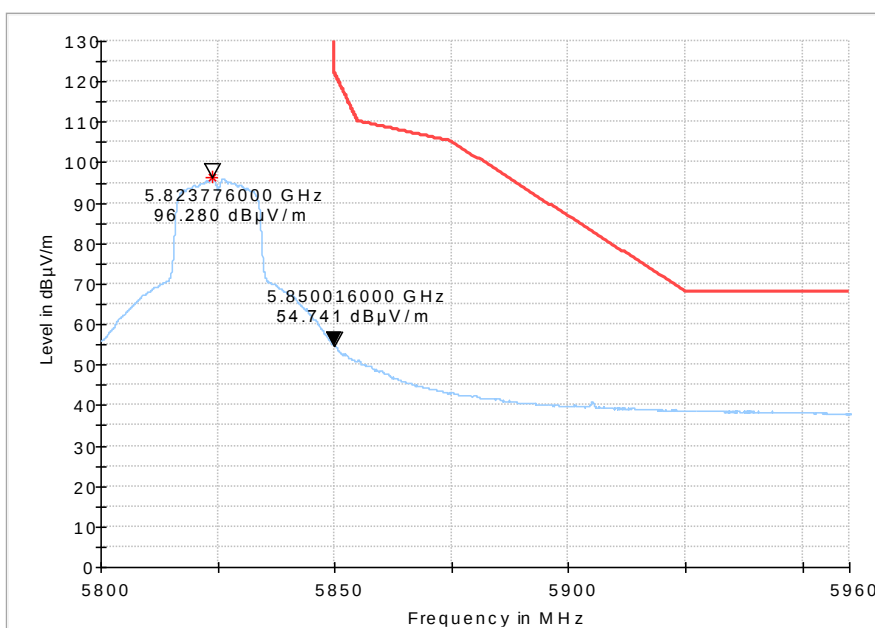
Fig. 76 Band Edges (802.11n-HT20, 5825MHz)
