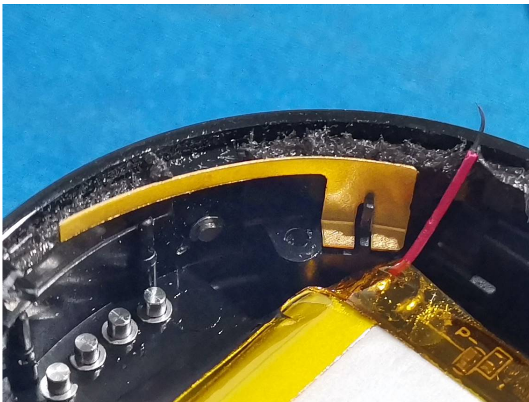
BLE/ANT+ Antenna
