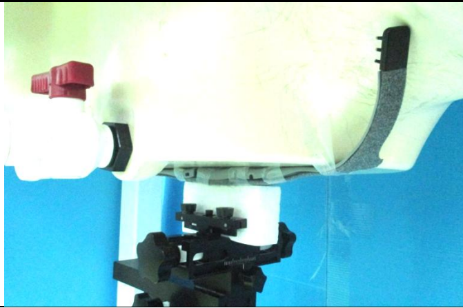
The EUT Surface of Antenna Location tested at 0 mm
