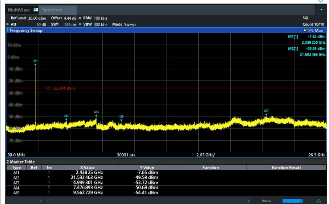
Tx. Spurious NVNT ax20 2437MHz Ant2 Emission
