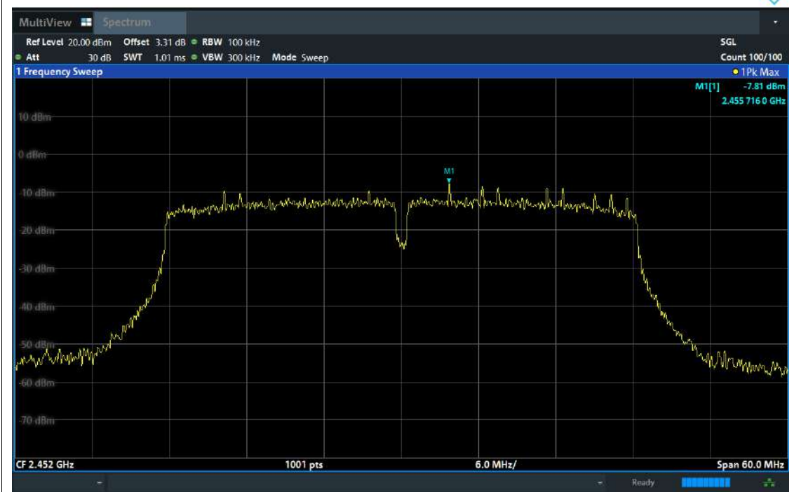
Tx. Spurious NVNT ax40 2452MHz Ant1 Emission
