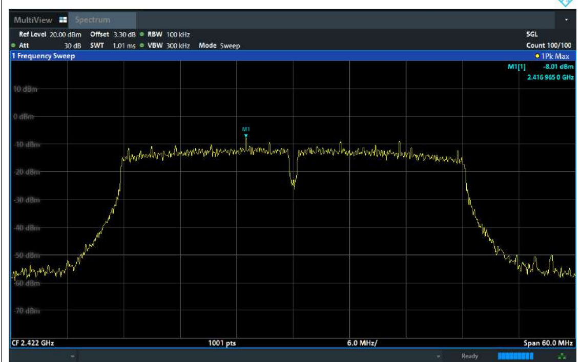
Tx. Spurious NVNT ax40 2422MHz Ant1 Emission
