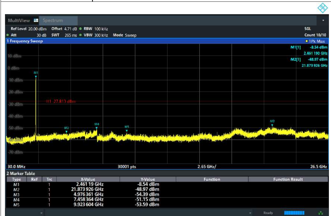
Tx. Spurious NVNT ax40 2452MHz Ant1 Emission
