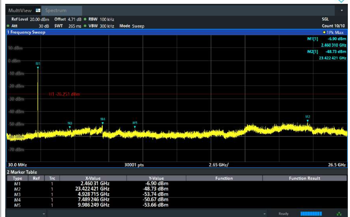
Tx. Spurious NVNT ax20 2462MHz Ant1 Emission
