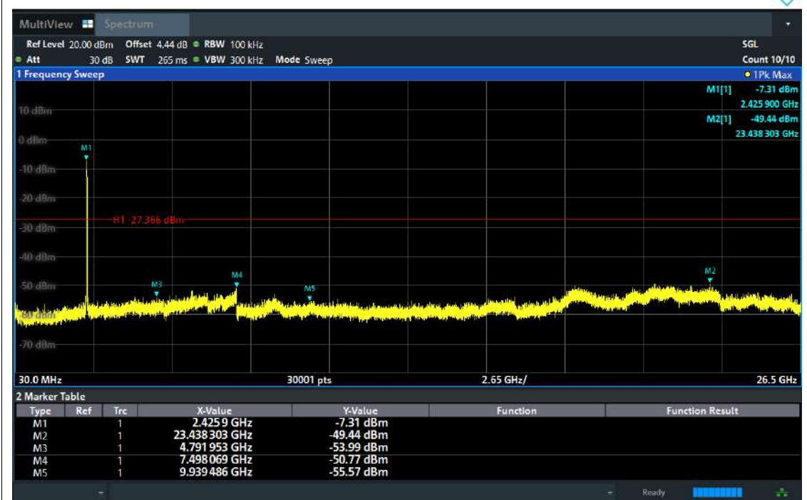
Tx. Spurious NVNT ax40 2437MHz Ant2 Emission
