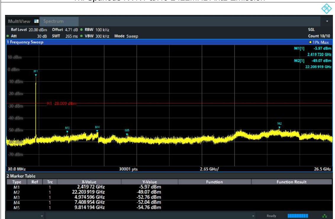
Tx. Spurious NVNT ax40 2422MHz Ant1 Emission
