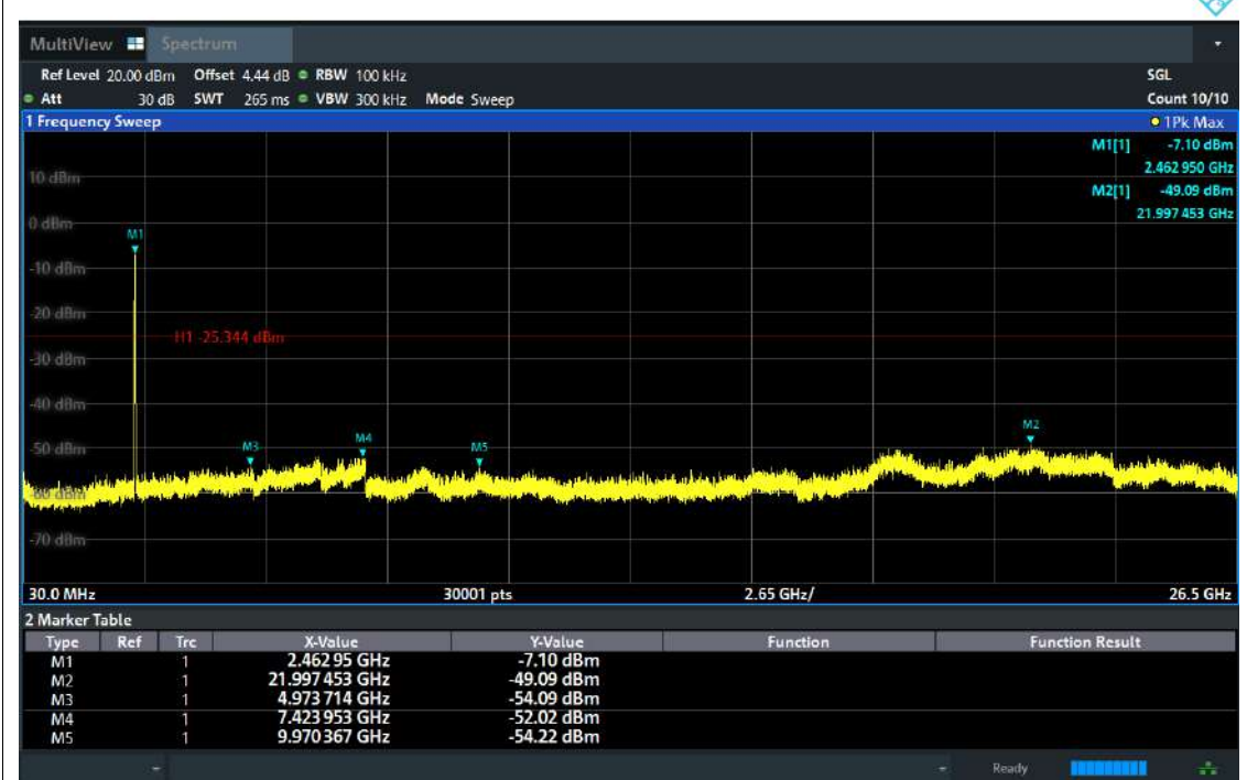
Tx. Spurious NVNT ax20 2462MHz Ant2 Emission
