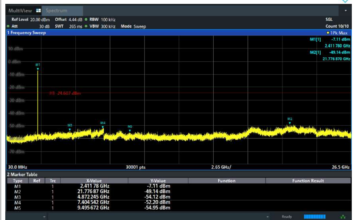
Tx. Spurious NVNT ax20 2412MHz Ant2 Emission
