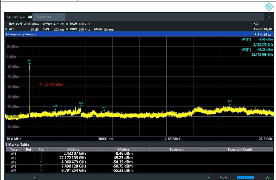
Tx. Spurious NVNT ax40 2437MHz Ant1 Emission
