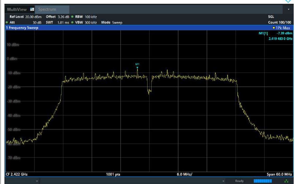
Tx. Spurious NVNT ax40 2422MHz Ant2 Emission
