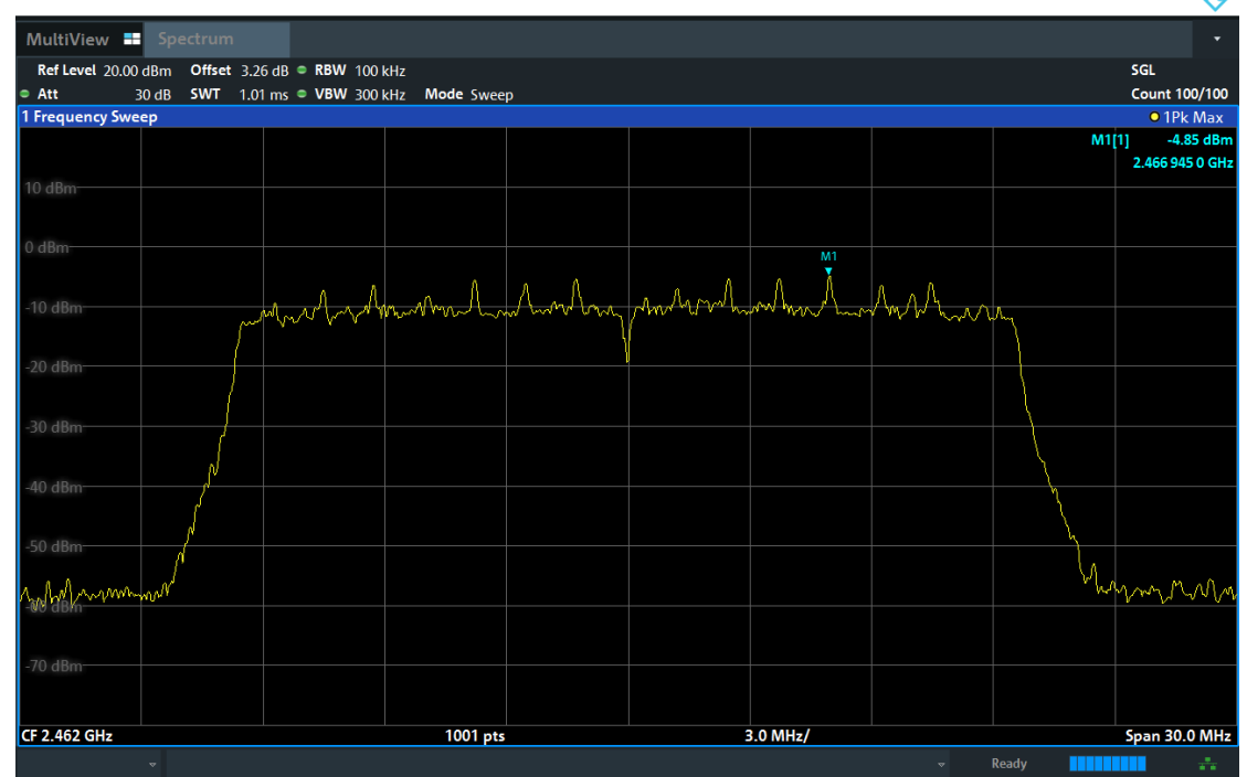
Band Edge NVNT ax20 2462MHz Ant2 Emission
