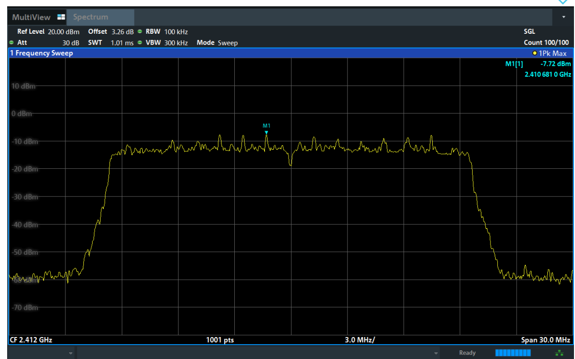
Band Edge NVNT ax20 2412MHz Ant2 Emission
