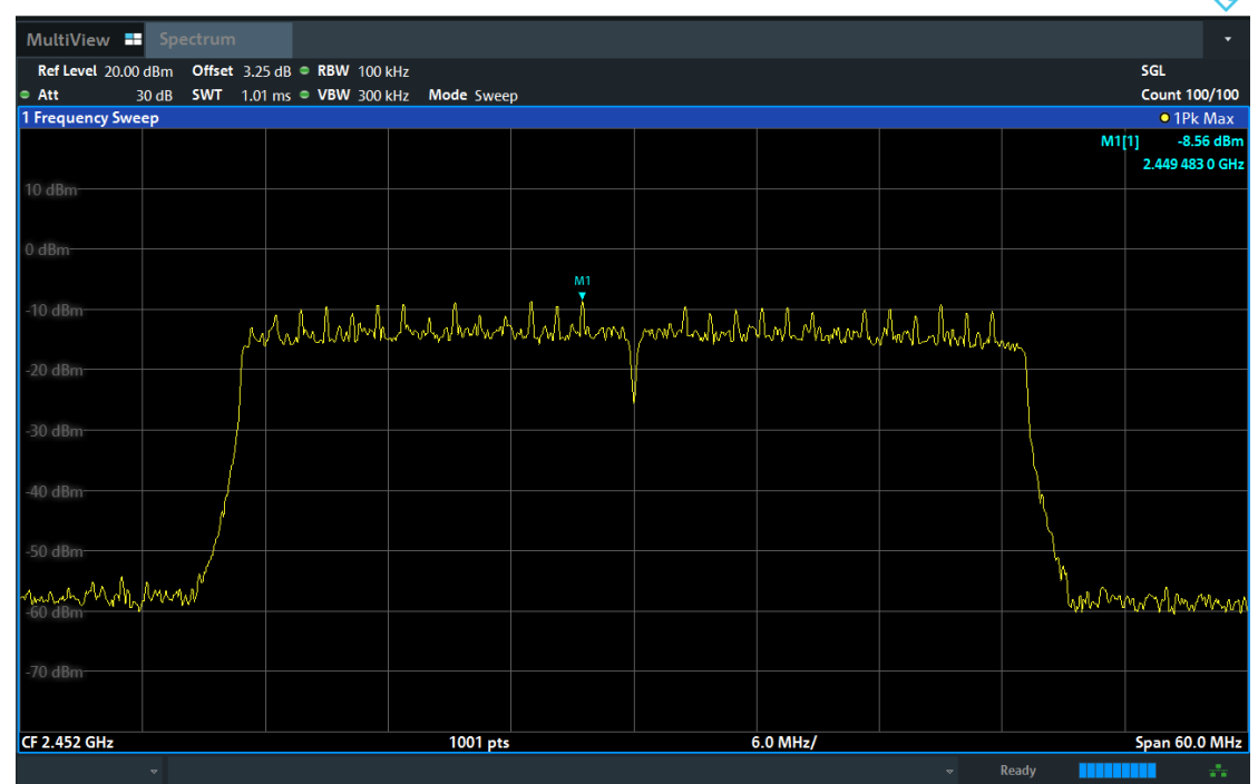
Band Edge NVNT ax40 2452MHz Ant2 Emission
