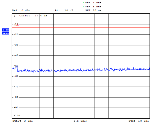
LTE Band 4 1.4MHz CH-Middle 3GHz~18GHz
