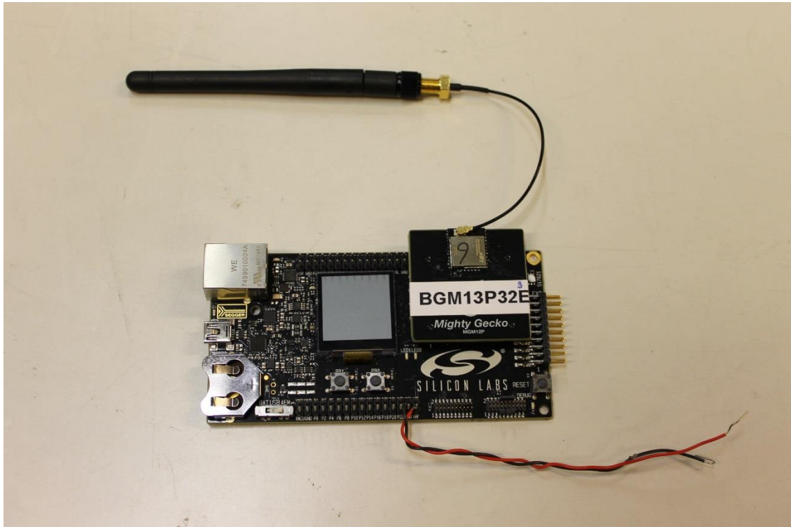
Photograph 3. DUT 3
