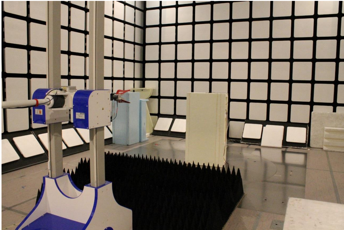
Photograph 7. Radiated Spurious Emissions 1 – 18 GHz
