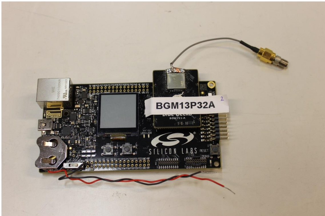
Photograph 2. DUT 2
