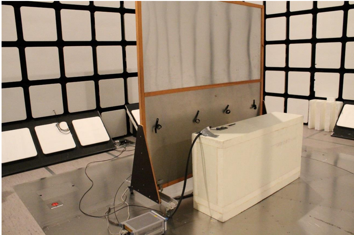
Photograph 11. Conducted Emissions
