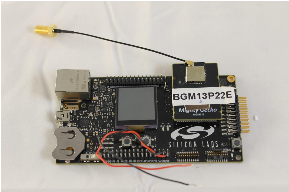
Photograph 5. DUT 5
