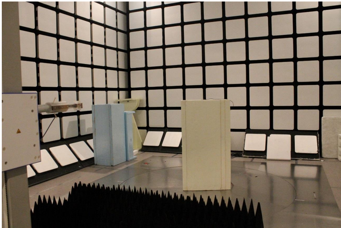
Photograph 8. Radiated Spurious Emissions 18 – 26.5 GHz
