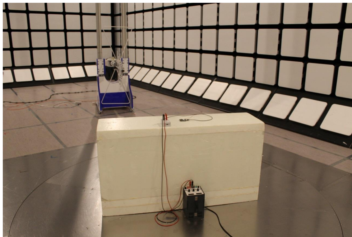
Photograph 10. EUT on table (integral chip antenna)
