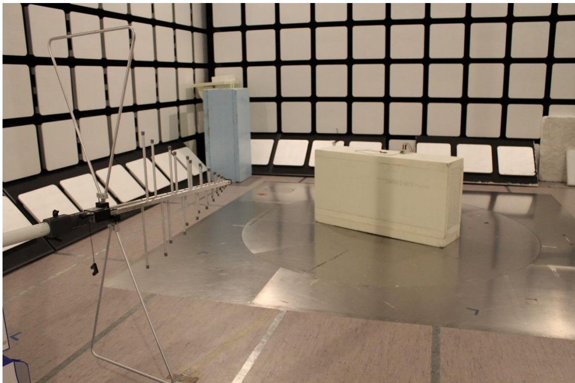
Photograph 6. Radiated Spurious Emissions 30 – 1000 MHz
