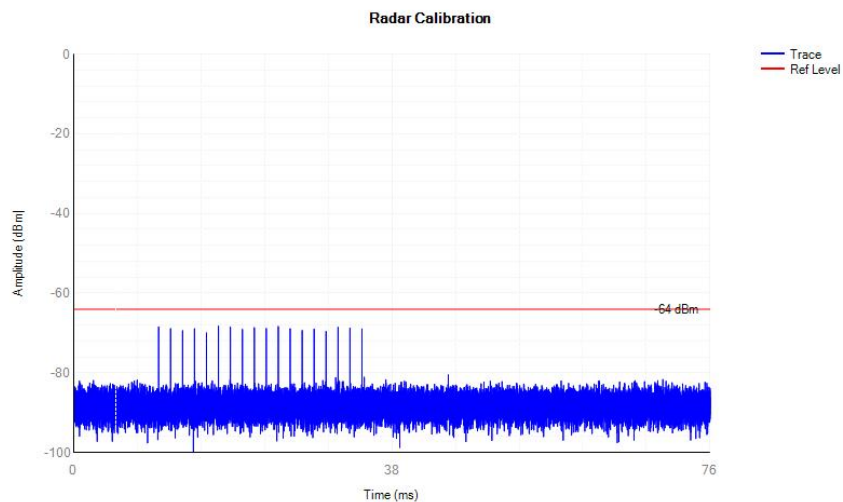
Signal Calibration_802.11ac(HT80)_2C_5530MHz_RadarType0_Trial0
