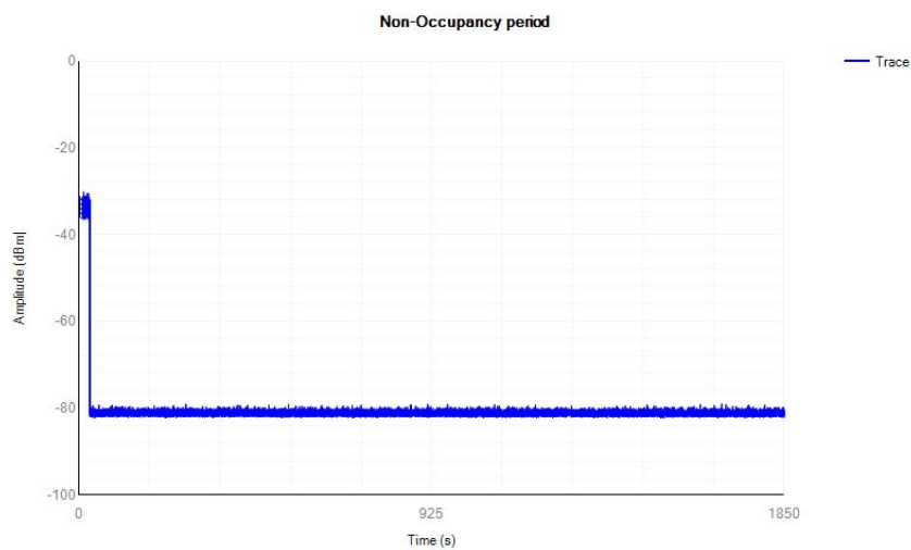
Non-Occupancy Period_802.11ac(HT80)_2C_5530MHz
