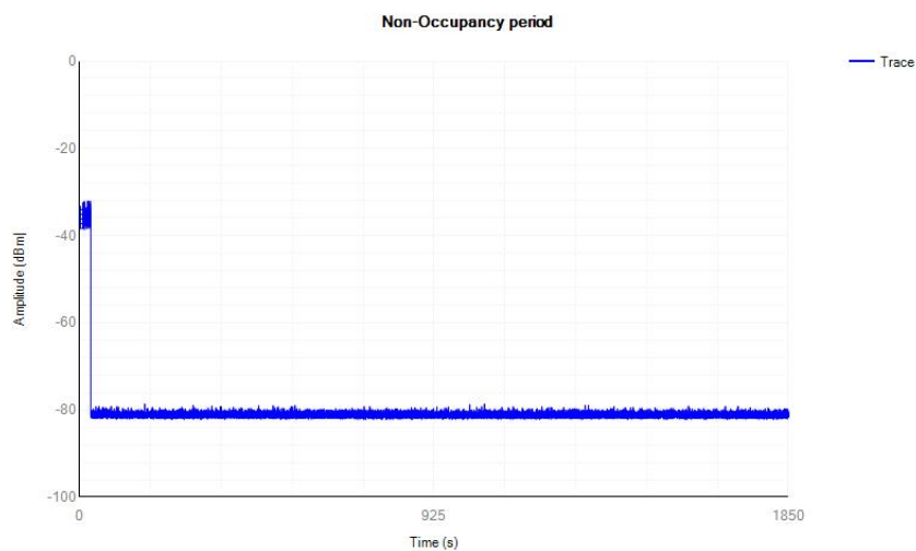
Non-Occupancy Period_802.11ac(HT80)_2C_5530MHz
