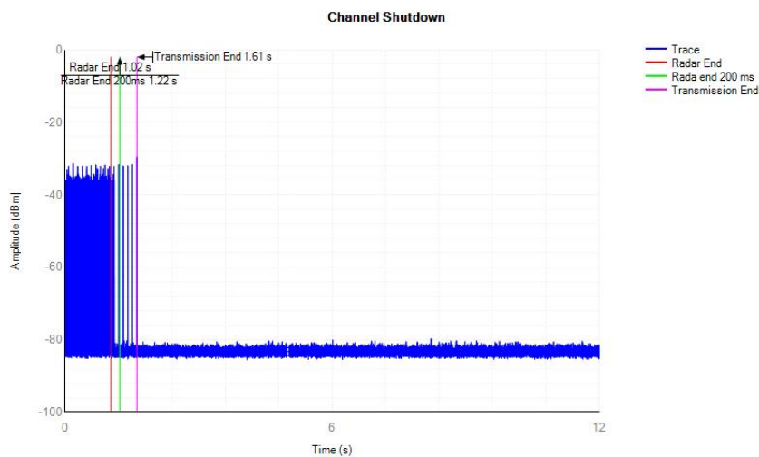
Channel Move Time and Closing Transmission Time_802.11ac(HT80)_2C_5530MHz
