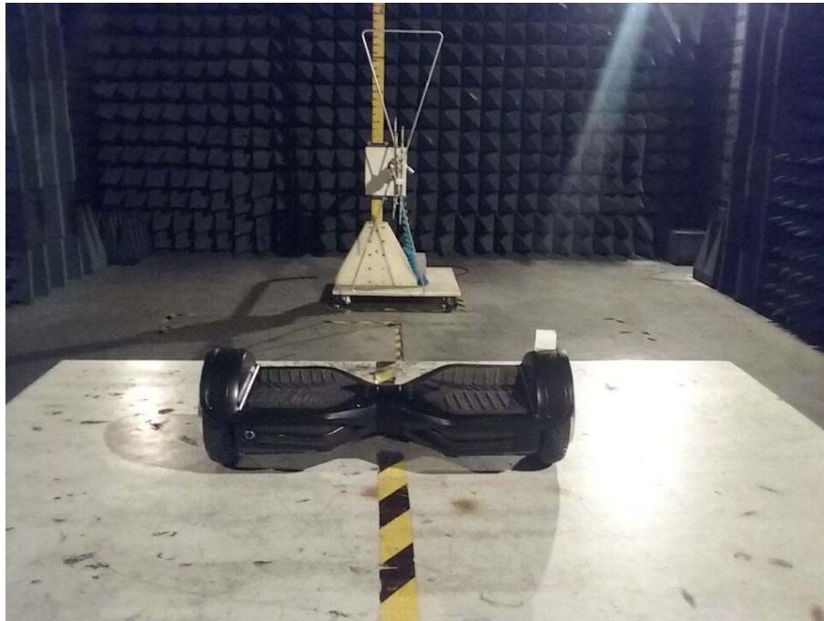
Below 1G-TYPE 2
