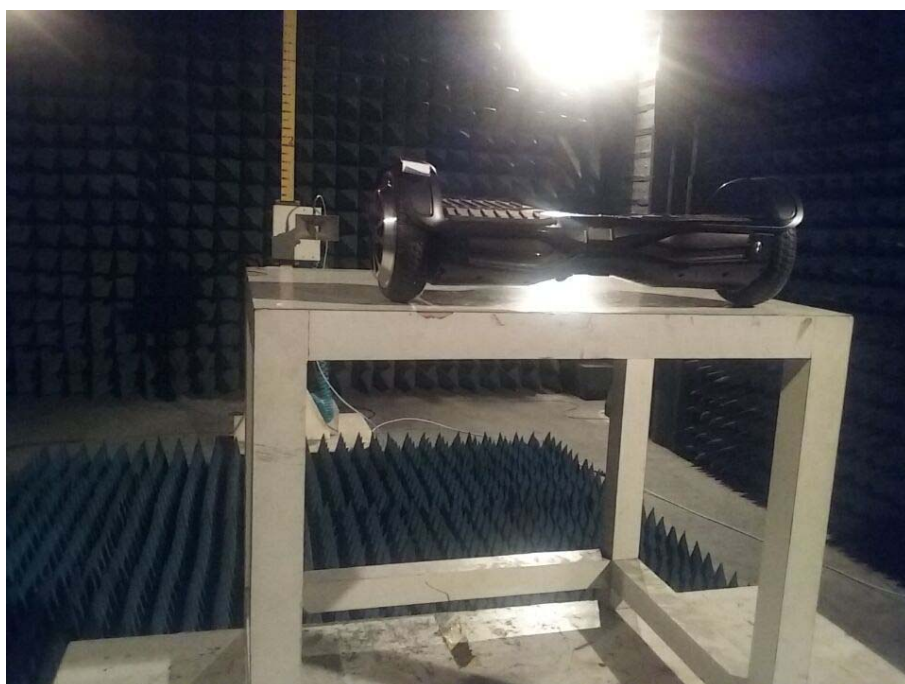
Above 1G-TYPE 2
