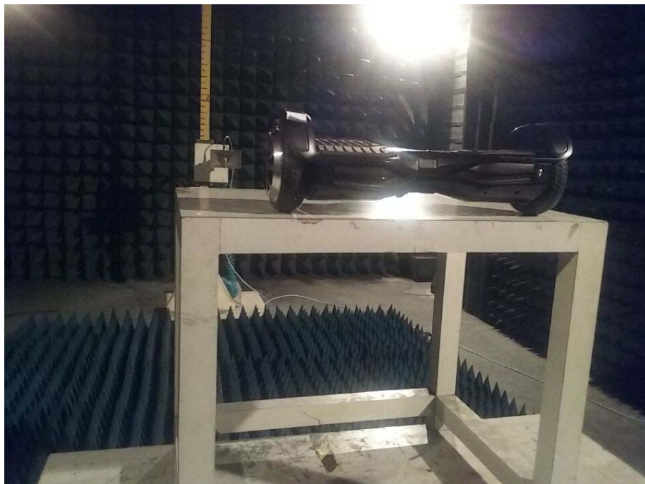
Above 1G-TYPE 2
