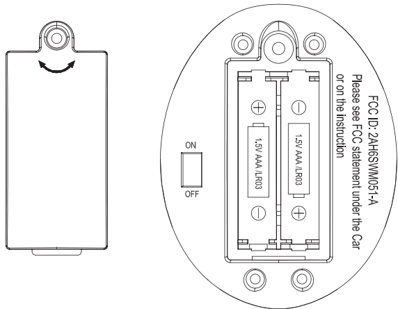
FIG. 1 REMOTE CONTROL POWER SWITCH & BATTERY COMPARTMENT
