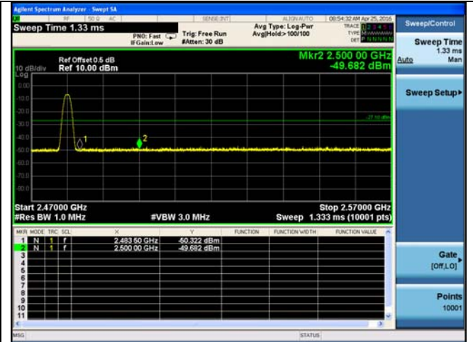
2480 MHz – Peak
