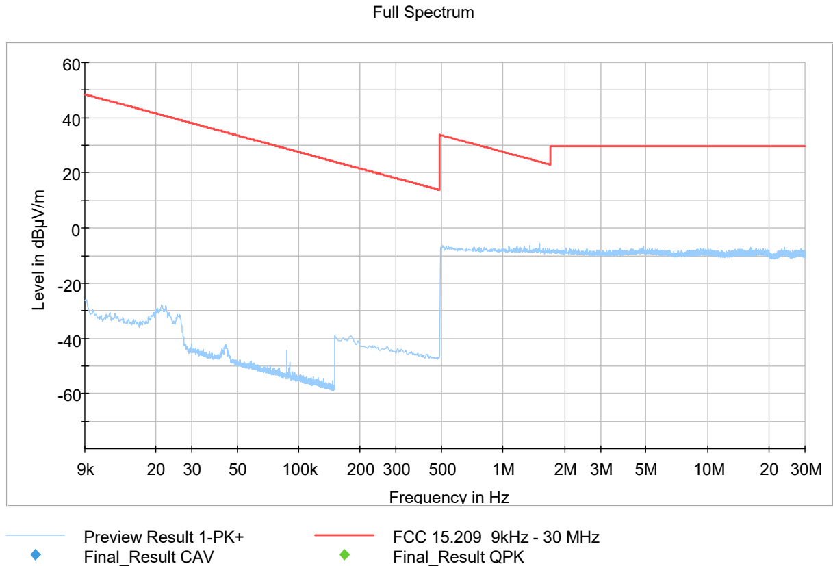
Figure 5: 9 kHz – 30 MHz, channel low
