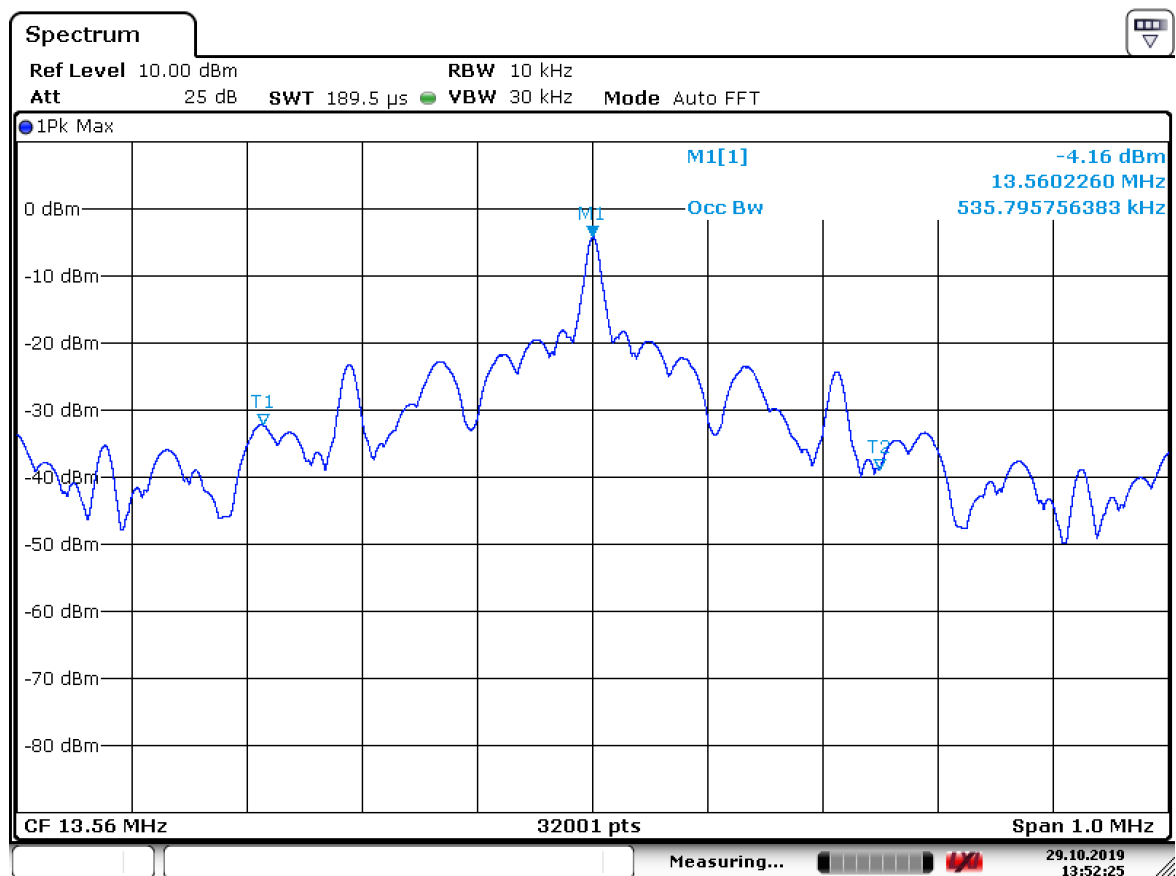
Figure 9. 99% Power Bandwidth
