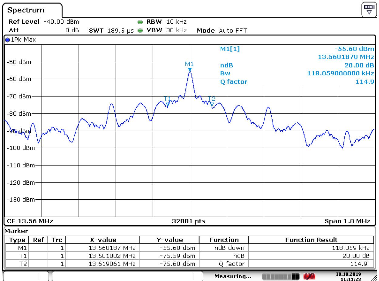
Figure 8: 20 dB bandwidth
