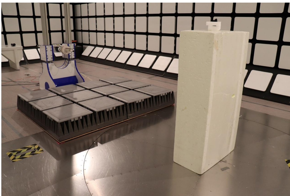
Photograph 4. Radiated Spurious Emissions 18 – 26.5 MHz
