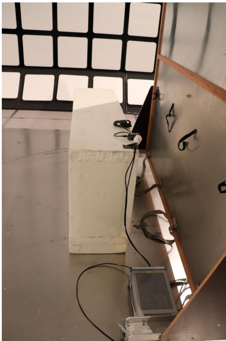
Photograph 3. Conducted emissions 0.15 – 30 MHz
