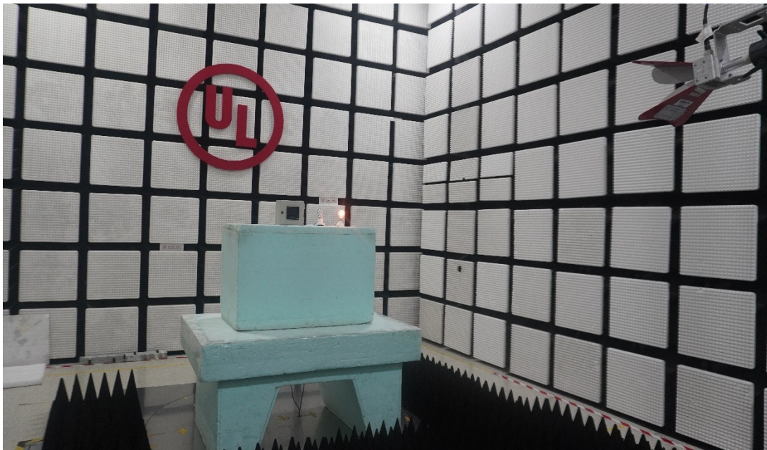
Radiated Emission_1GHz to 18GHz_Vertical Polarization
