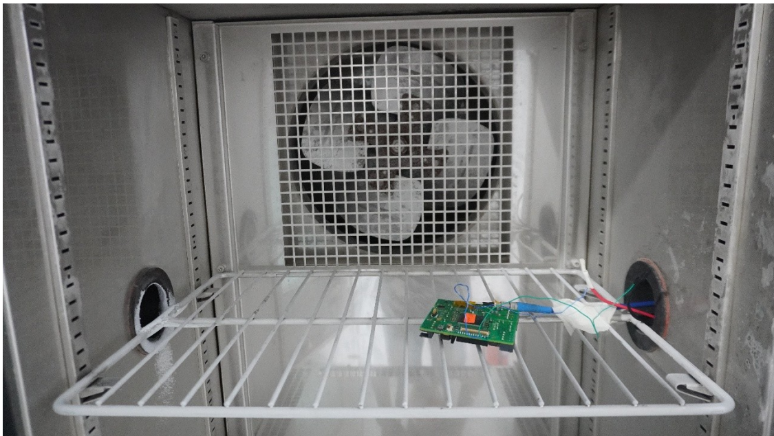
Test Setup_Conducted RF _ Extreme Condition using thermal chamber.
