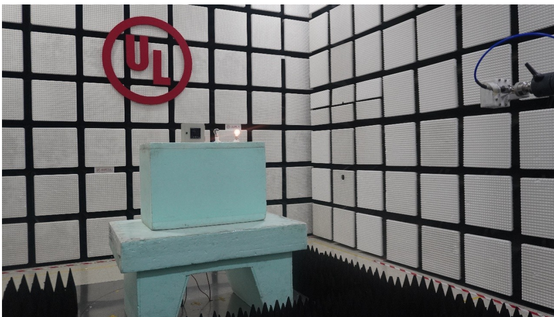
Radiated Emission_18GHz to 26.5GHz_Horizontal Polarization
