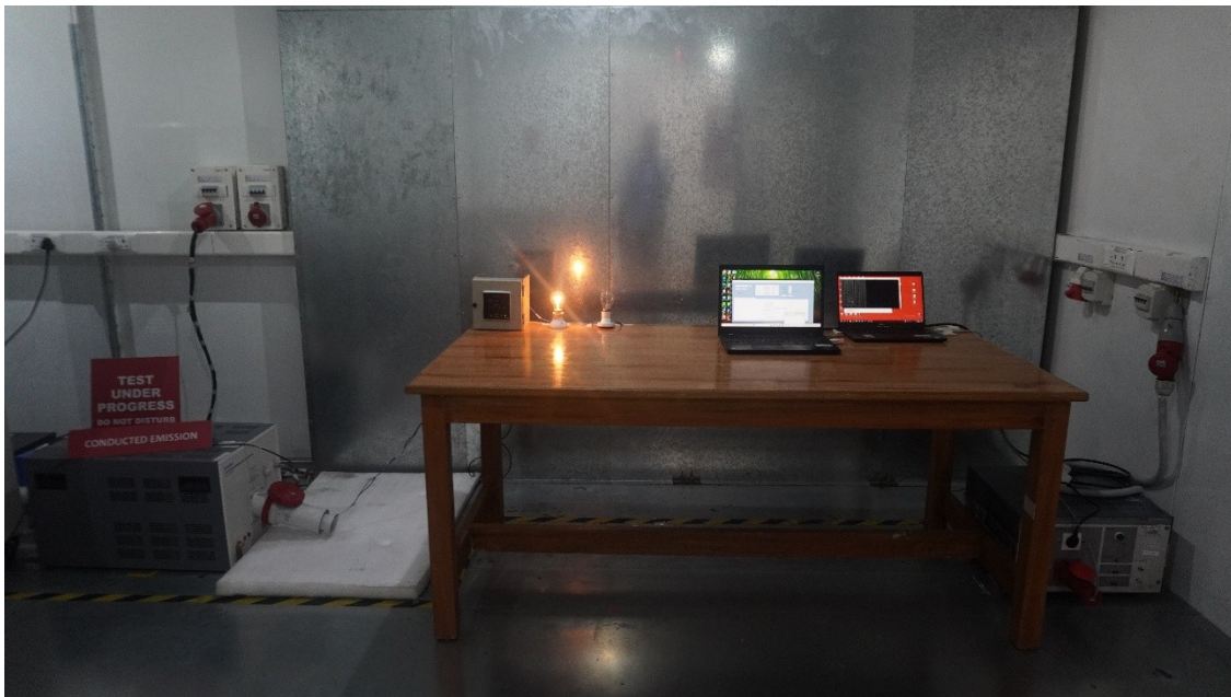
Conducted Emission_150kHz to 30MHz
