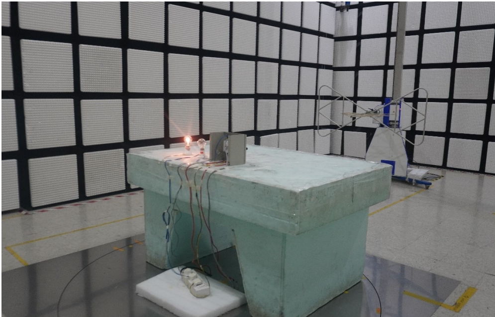
Radiated Emission_30MHz to 1 GHz_Horizontal Polarization
