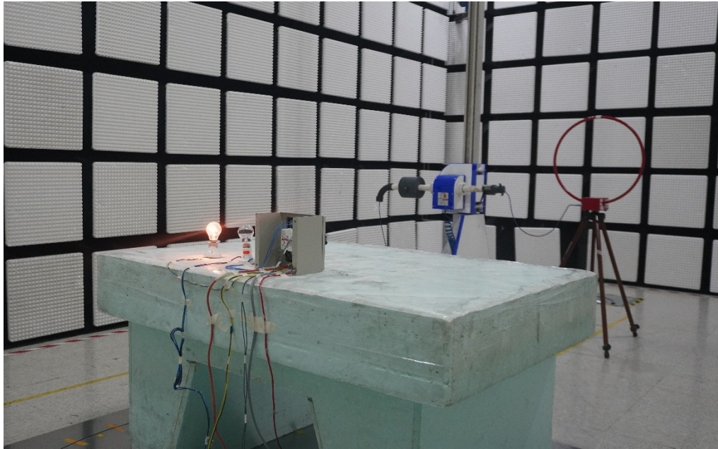
Radaited Emission_9kHz to 30MHz_Loop antenna in Parallel
