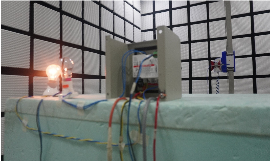
Radiated Emission_1GHz to 18GHz_Horizontal Polarization
