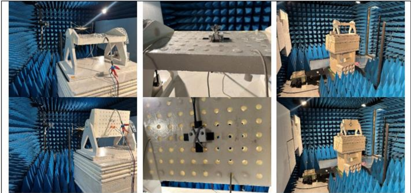
Photo of Unwanted Emissions in Restricted Frequency Bands
