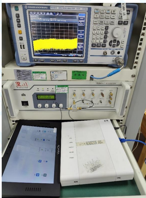
Photo of Setup for DFS Test
