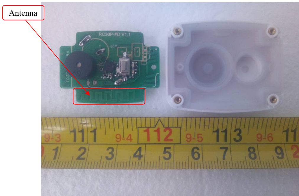
EUT –Cover off View 2
