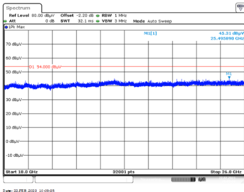
Plot 7: 18 GHz to 26 GHz, TX mode, vertical & horizontal polarization, valid for all channels and modes
