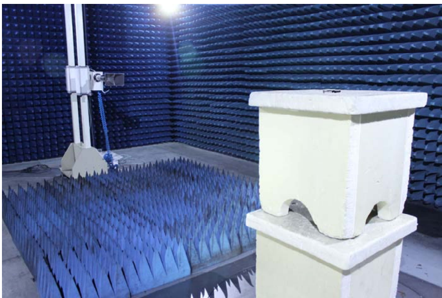
Photograph of set-up for Radiated Emission above 1GHz
