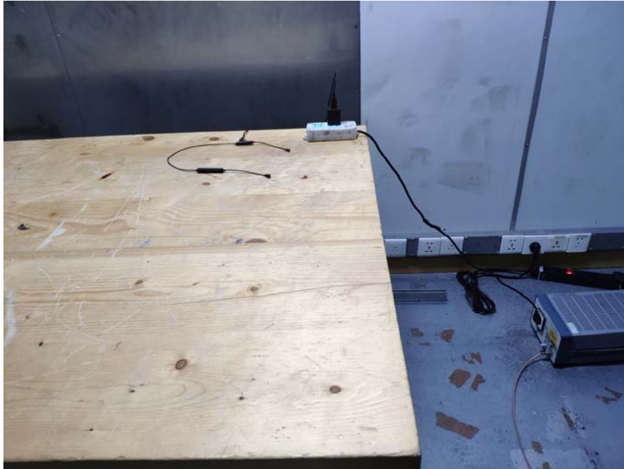
Photograph of set-up for ac power line Conducted emission
