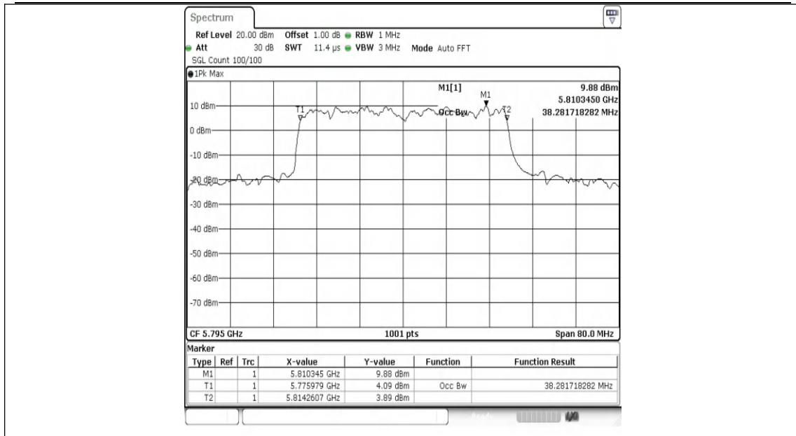
11AX40SISO-Ant1-5795
