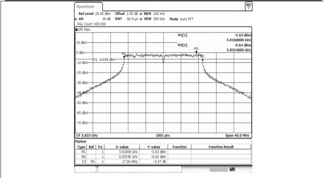
11AC20SISO-Ant1-5825-PASS
