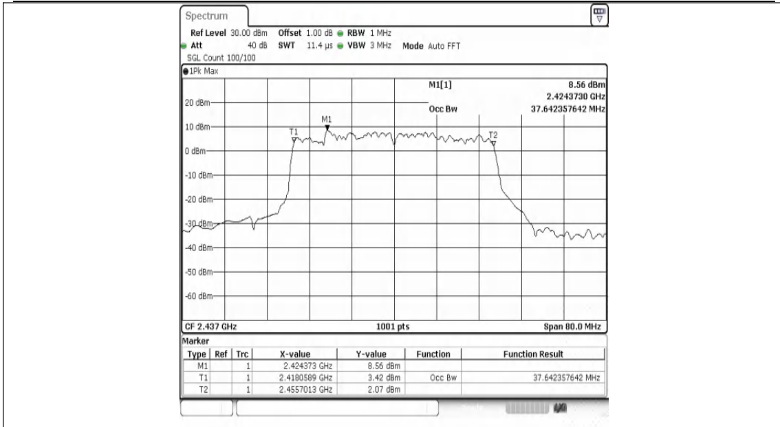
11AX40SISO-Ant1-2437
