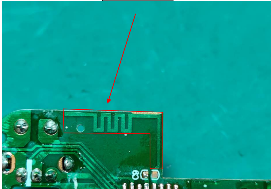
ANT- BT&BLE
