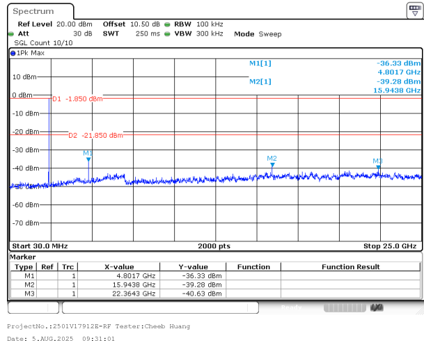
BLE_2M_High_Channel
