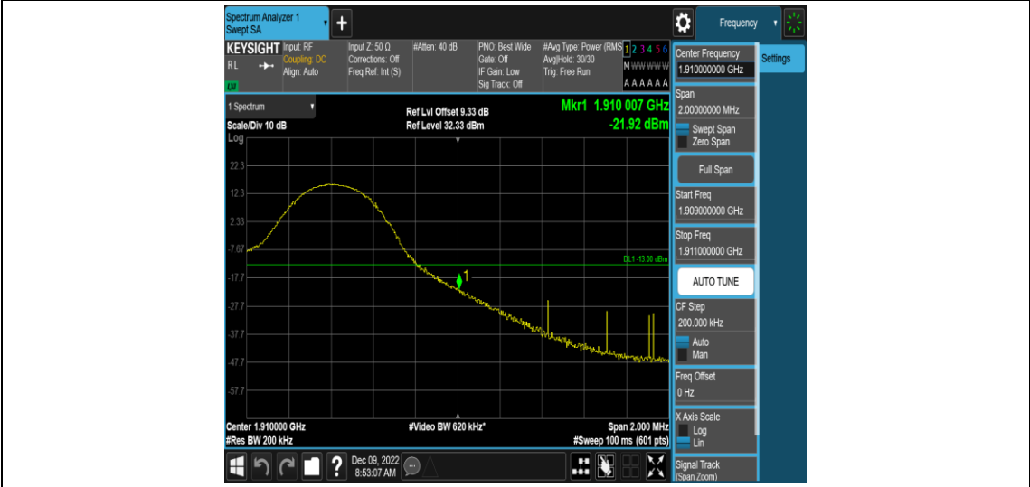
Band2-10MHz-QPSK-19150-50RB#0
