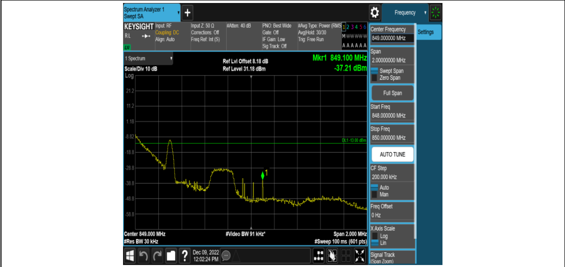
Band5-1.4MHz-QPSK-20643-1RB#5
