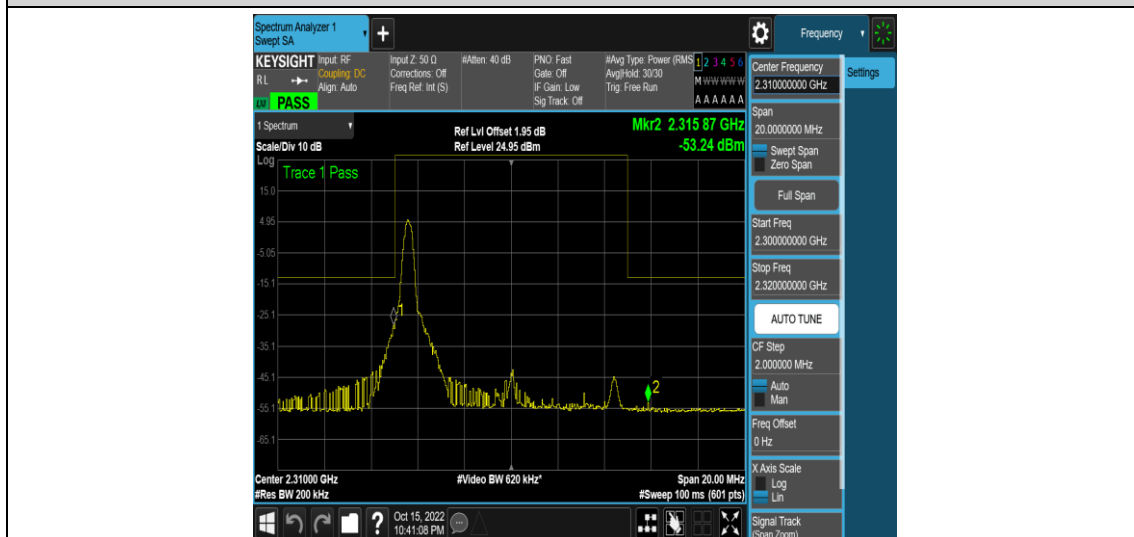
Band40-10MHz-16QAM-38750-1RB#49
