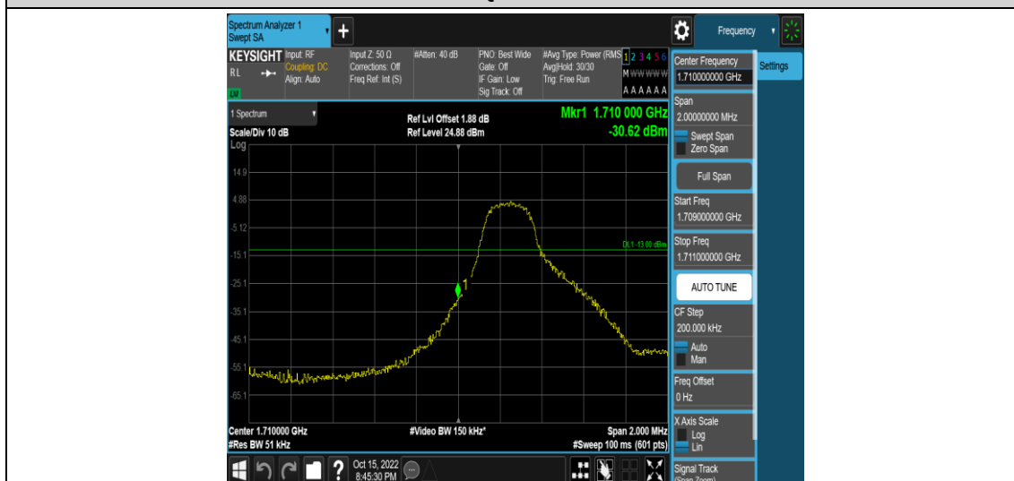
Band66-3MHz-QPSK-131987-1RB#14
