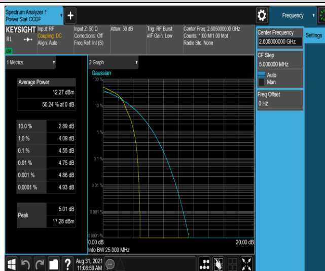
Band41-20MHz-16QAM-40740-100RB#0
