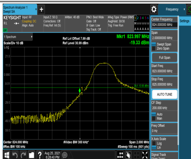
Band5-5MHz-16QAM-20425-1RB#24
