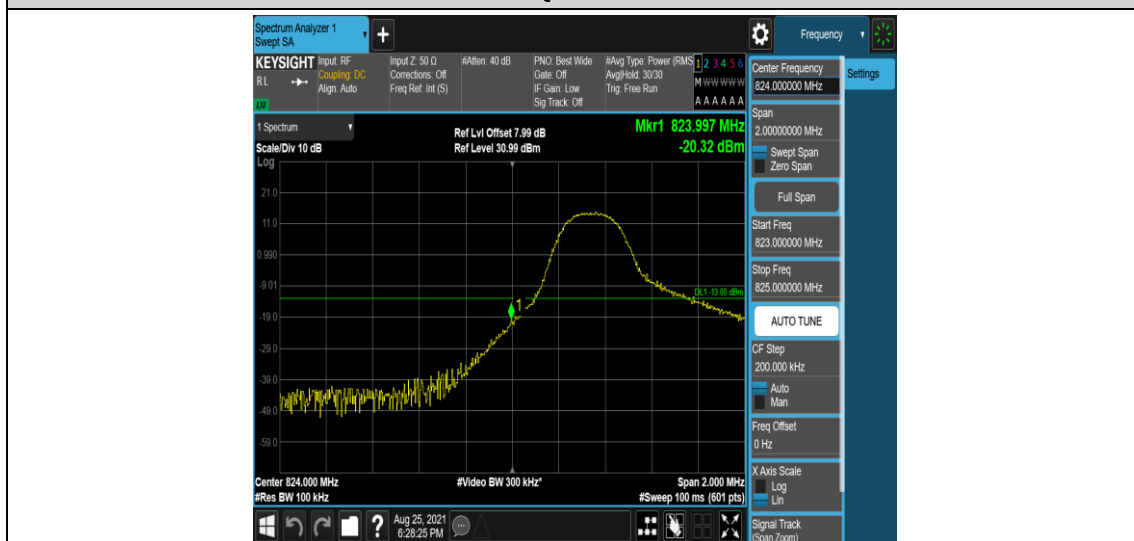
Band5-5MHz-QPSK-20425-1RB#24
