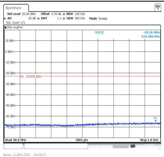
Band4_1.4MHz_16QAM_19957_1RB#0_30~1000_30~1000
