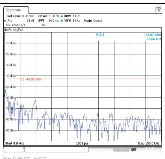
Band4_1.4MHz_16QAM_19957_1RB#0_0.009~0.15_0.009~0.15
