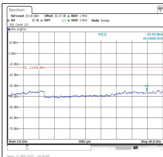
Band4_1.4MHz_QPSK_19957_1RB#0_3000~20000_3000~20000
