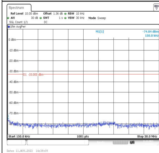
Band4_1.4MHz_16QAM_19957_1RB#0_0.15~30_0.15~30
