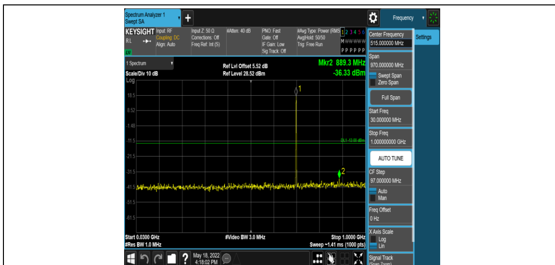
Band12-1.4MHz-QPSK-23095-1RB#0-Range3:30~1000MHz
