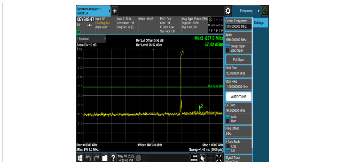
Band12-3MHz-QPSK-23095-1RB#0-Range3:30~1000MHz
