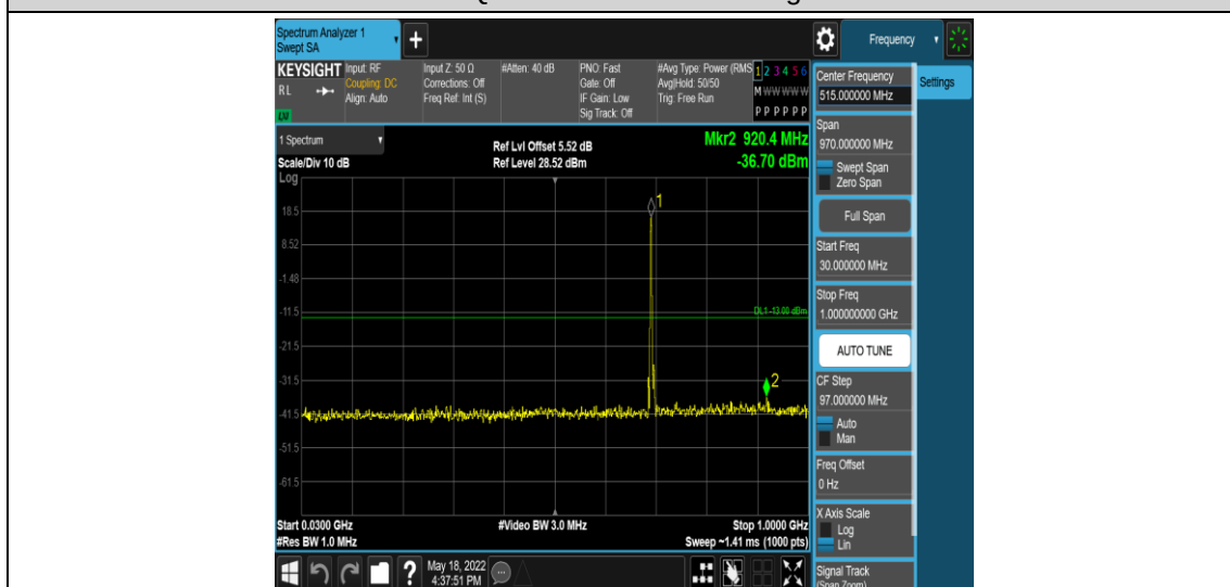
Band12-3MHz-16QAM-23025-1RB#0-Range3:30~1000MHz
