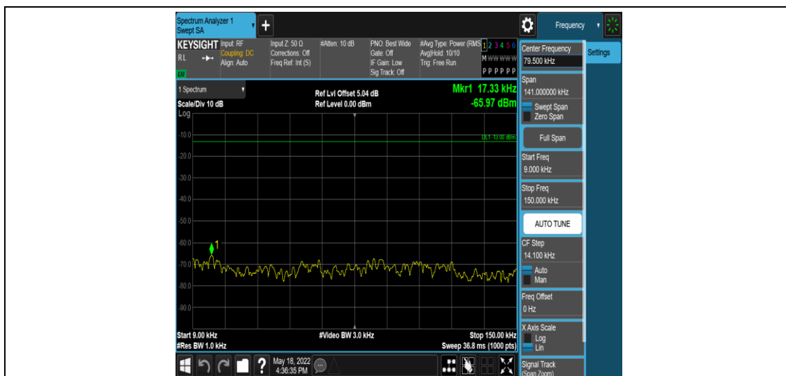
Band12-3MHz-QPSK-23025-1RB#0-Range1:0.009~0.15MHz
