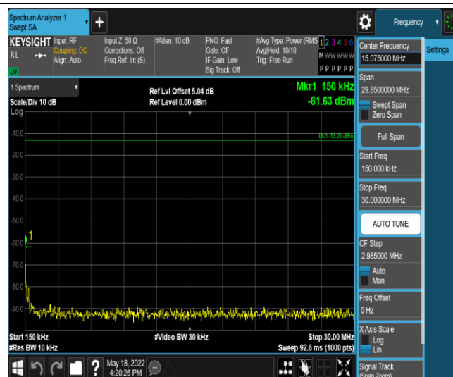
Band12-1.4MHz-16QAM-23173-1RB#0-Range2:0.15~30MHz
