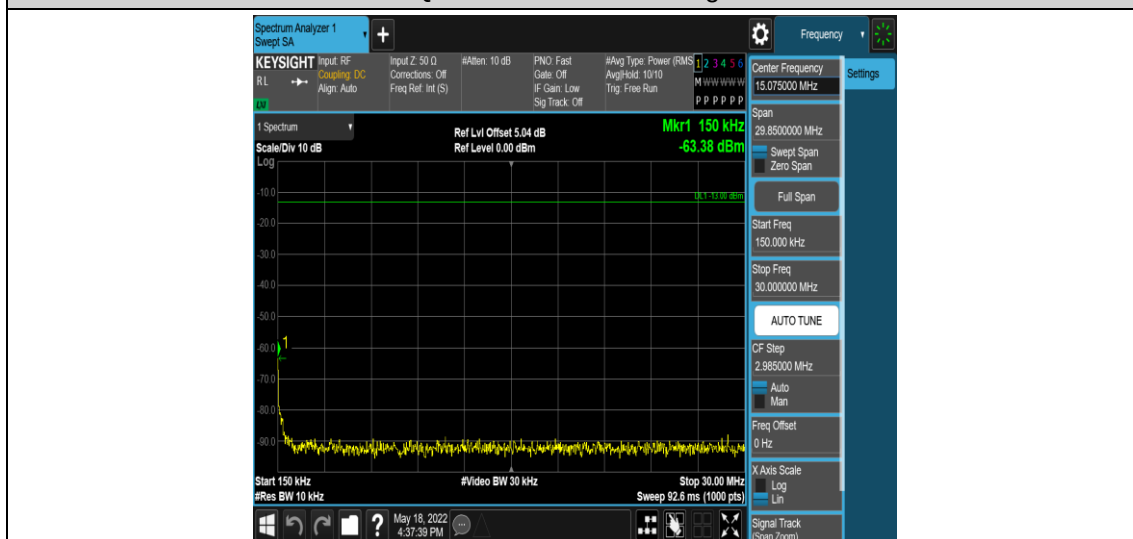
Band12-3MHz-16QAM-23025-1RB#0-Range2:0.15~30MHz
