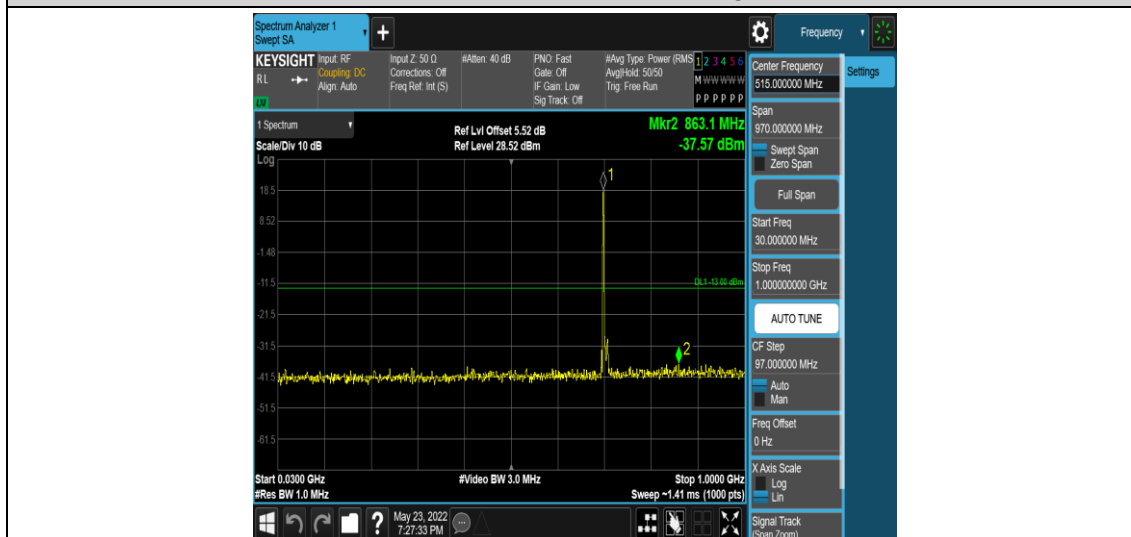
Band17-10MHz-16QAM-23800-1RB#0-Range3:30~1000MHz
