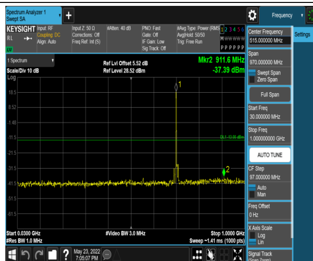
Band17-5MHz-QPSK-23790-1RB#0-Range3:30~1000MHz
