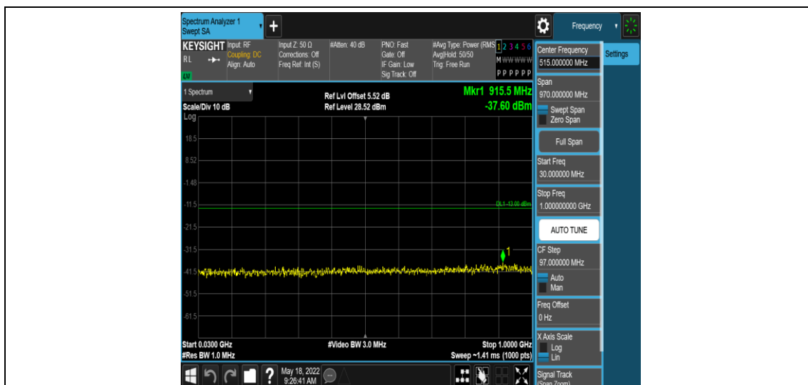
Band2-3MHz-16QAM-18900-1RB#0-Range3:30~1000MHz
