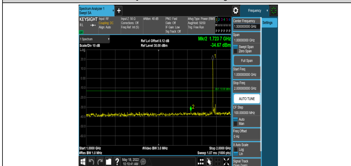
Band2-10MHz-16QAM-18900-1RB#0-Range4:1000~2000MHz
