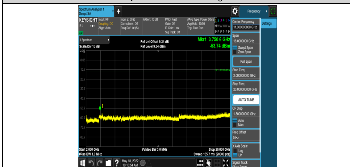
Band2-10MHz-16QAM-18900-1RB#0-Range5:2000~20000MHz
