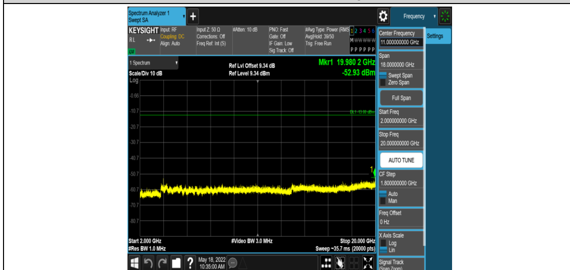
Band2-15MHz-16QAM-19125-1RB#0-Range5:2000~20000MHz
