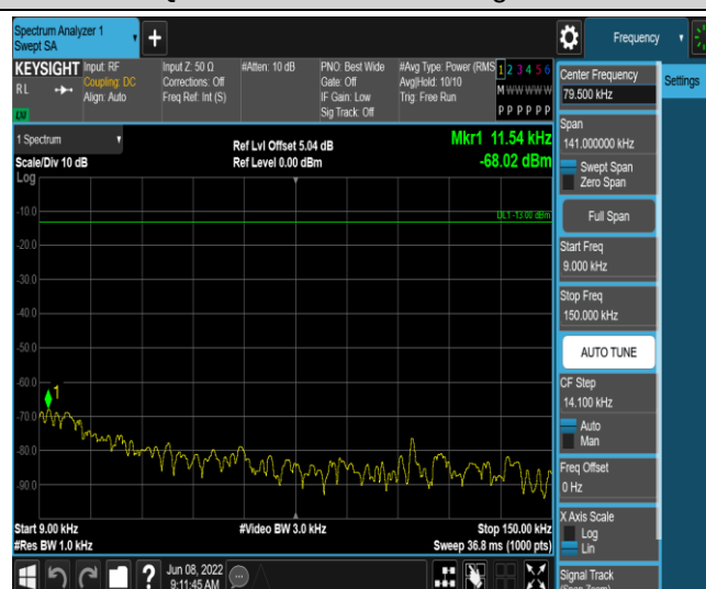
Band38-5MHz-QPSK-38225-1RB#0-Range1:0.009~0.15MHz
