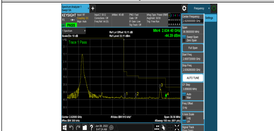
Band38-15MHz-16QAM-38175-1RB#0
