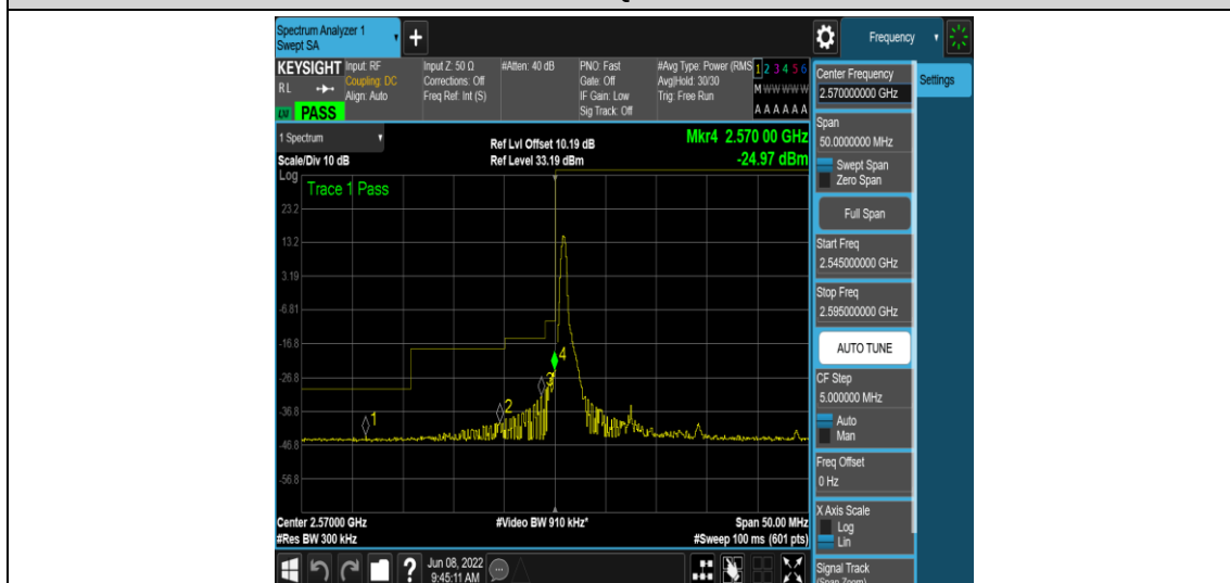
Band38-15MHz-QPSK-37825-1RB#0
