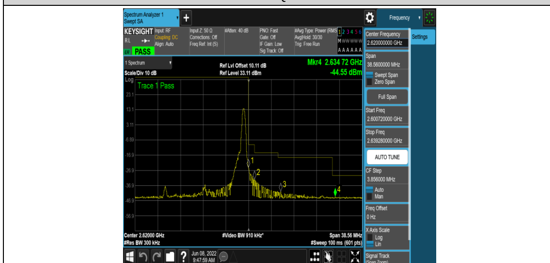
Band38-15MHz-16QAM-38175-1RB#74
