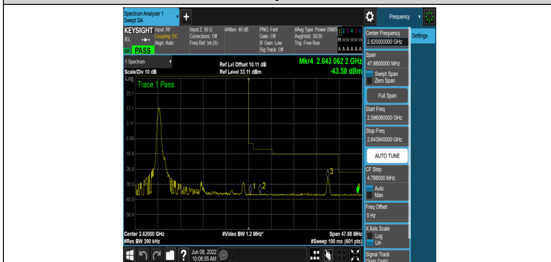
Band38-20MHz-16QAM-38150-1RB#0
