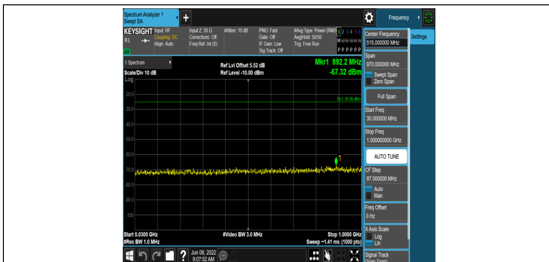
Band38-5MHz-QPSK-37775-1RB#0-Range3:30~1000MHz
