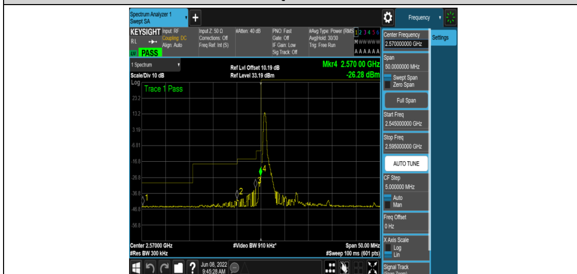
Band38-15MHz-16QAM-37825-1RB#0
