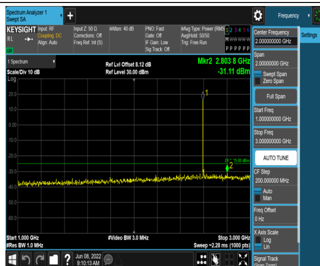
Band38-5MHz-QPSK-38000-1RB#0-Range4:1000~3000MHz
