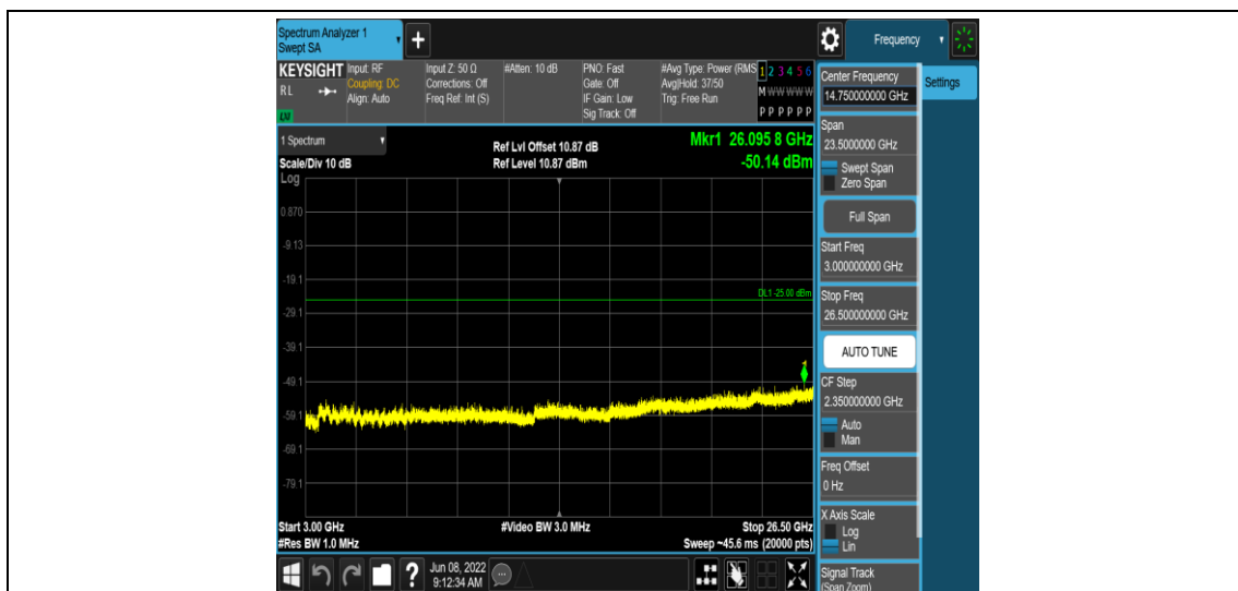
Band38-5MHz-QPSK-38225-1RB#0-Range5:3000~26500MHz
