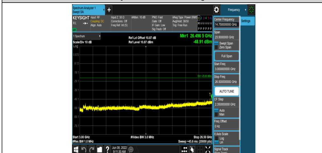
Band38-5MHz-16QAM-38000-1RB#0-Range5:3000~26500MHz
