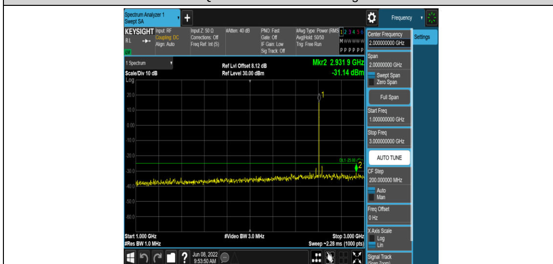
Band38-15MHz-QPSK-38175-1RB#0-Range4:1000~3000MHz
