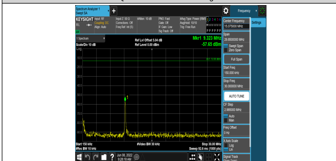
Band38-10MHz-QPSK-37800-1RB#0-Range2:0.15~30MHz
