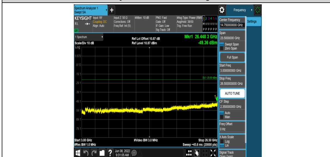
Band38-10MHz-QPSK-38000-1RB#0-Range5:3000~26500MHz
