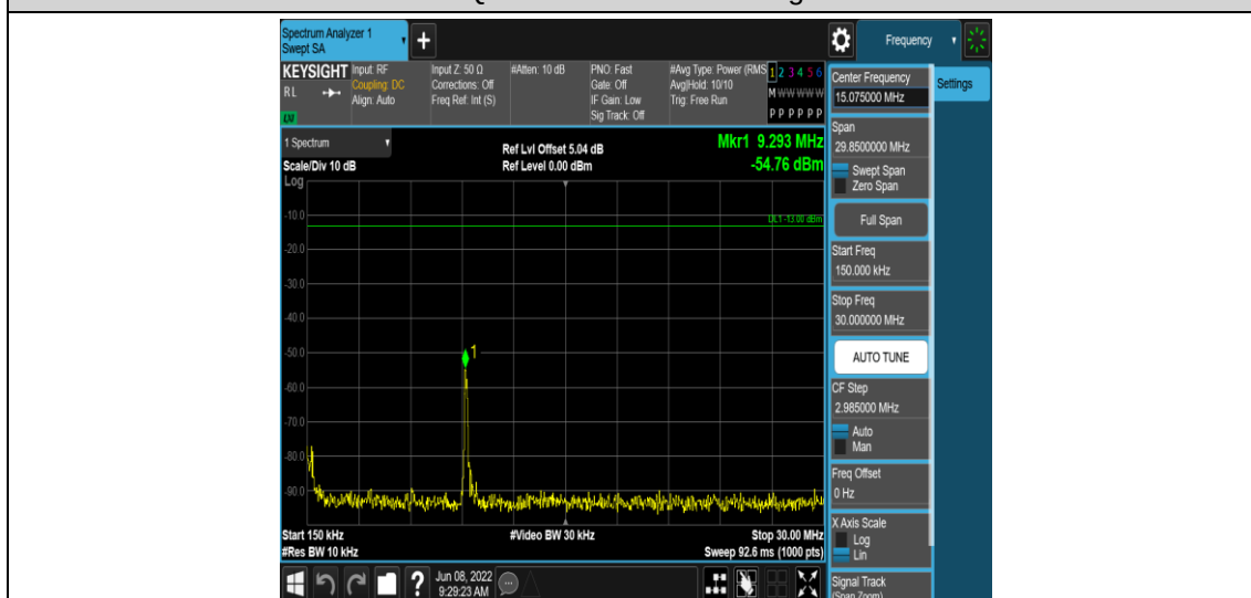
Band38-10MHz-16QAM-37800-1RB#0-Range2:0.15~30MHz
