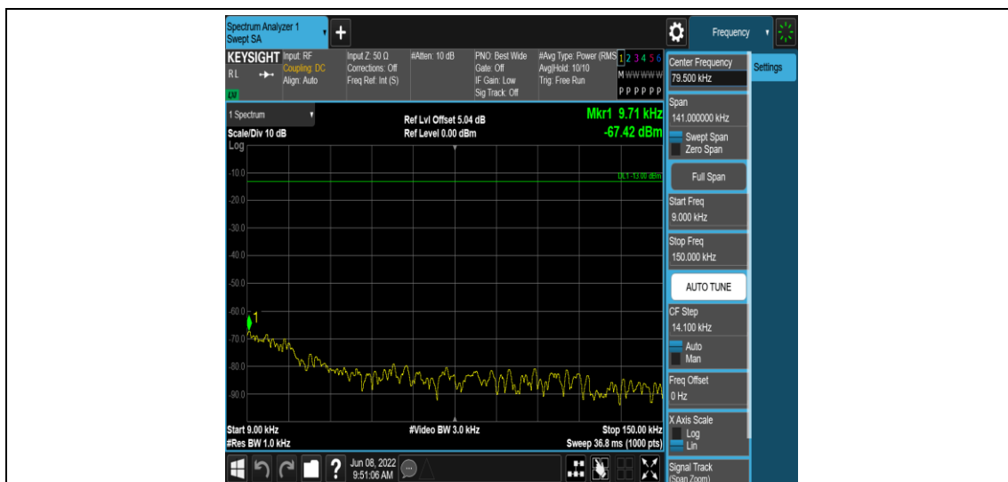
Band38-15MHz-QPSK-38000-1RB#0-Range1:0.009~0.15MHz
