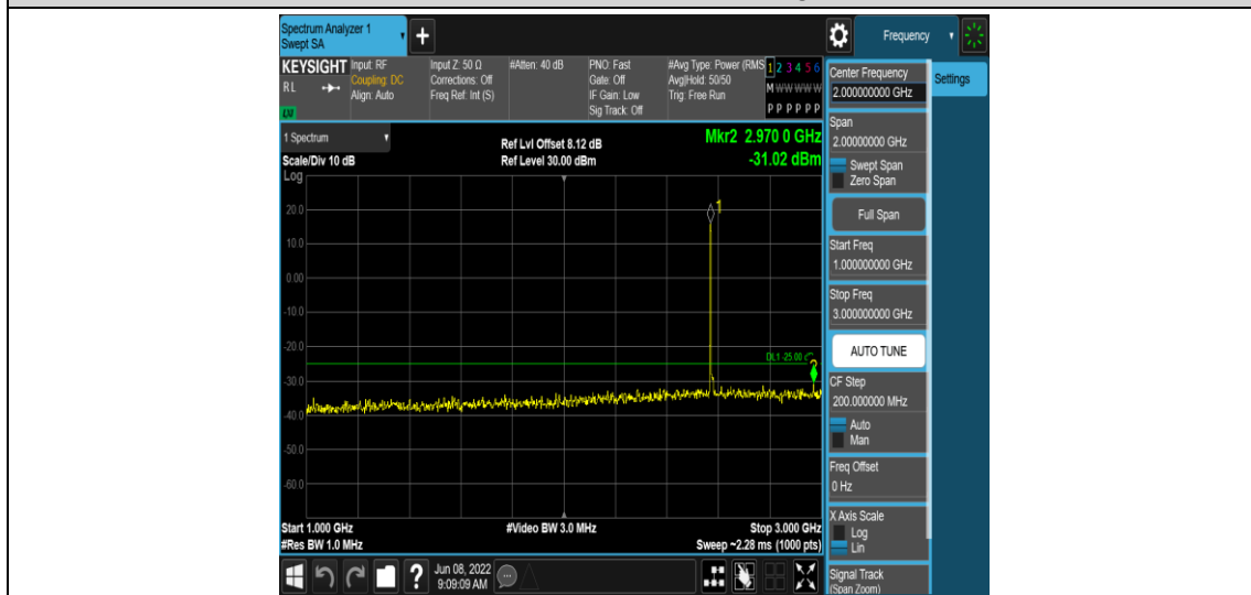
Band38-5MHz-16QAM-37775-1RB#0-Range4:1000~3000MHz
