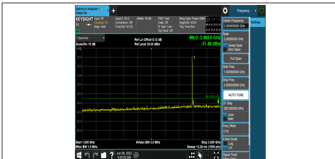
Band38-10MHz-QPSK-38000-1RB#0-Range4:1000~3000MHz
