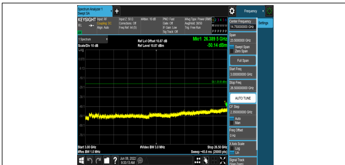
Band38-10MHz-QPSK-38200-1RB#0-Range5:3000~26500MHz
