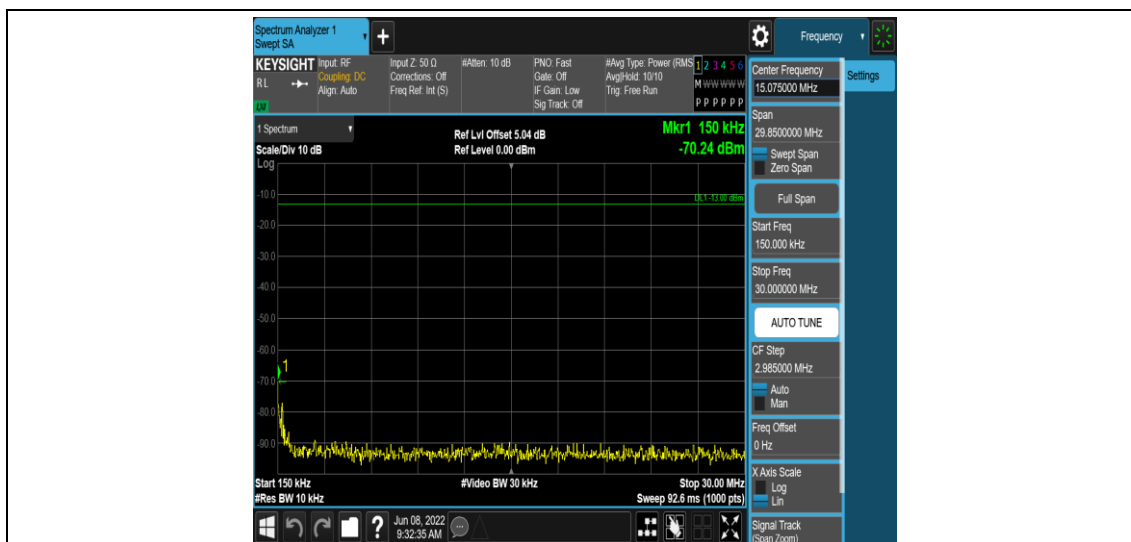
Band38-10MHz-QPSK-38200-1RB#0-Range2:0.15~30MHz
