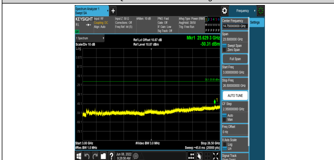
Band38-10MHz-QPSK-37800-1RB#0-Range5:3000~26500MHz
