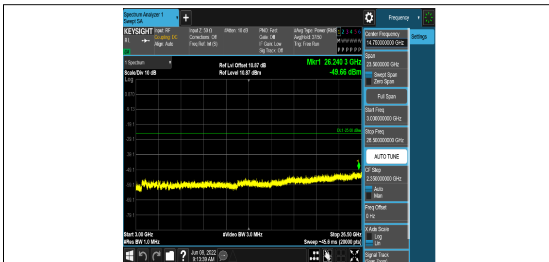
Band38-5MHz-16QAM-38225-1RB#0-Range5:3000~26500MHz
