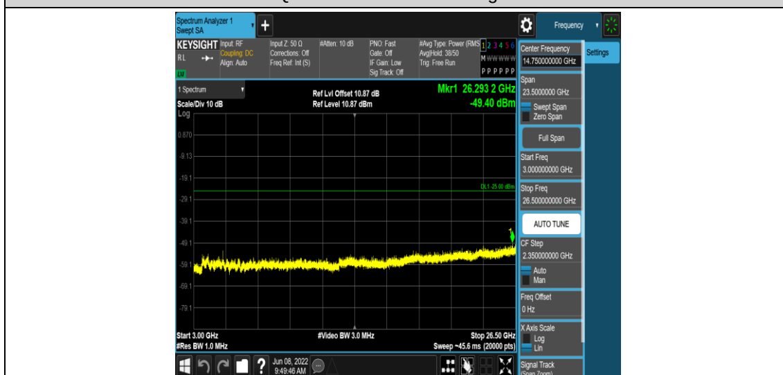
Band38-15MHz-QPSK-37825-1RB#0-Range5:3000~26500MHz
