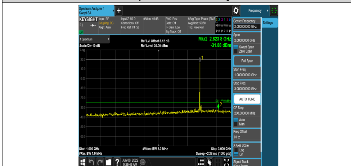
Band38-10MHz-16QAM-37800-1RB#0-Range4:1000~3000MHz
