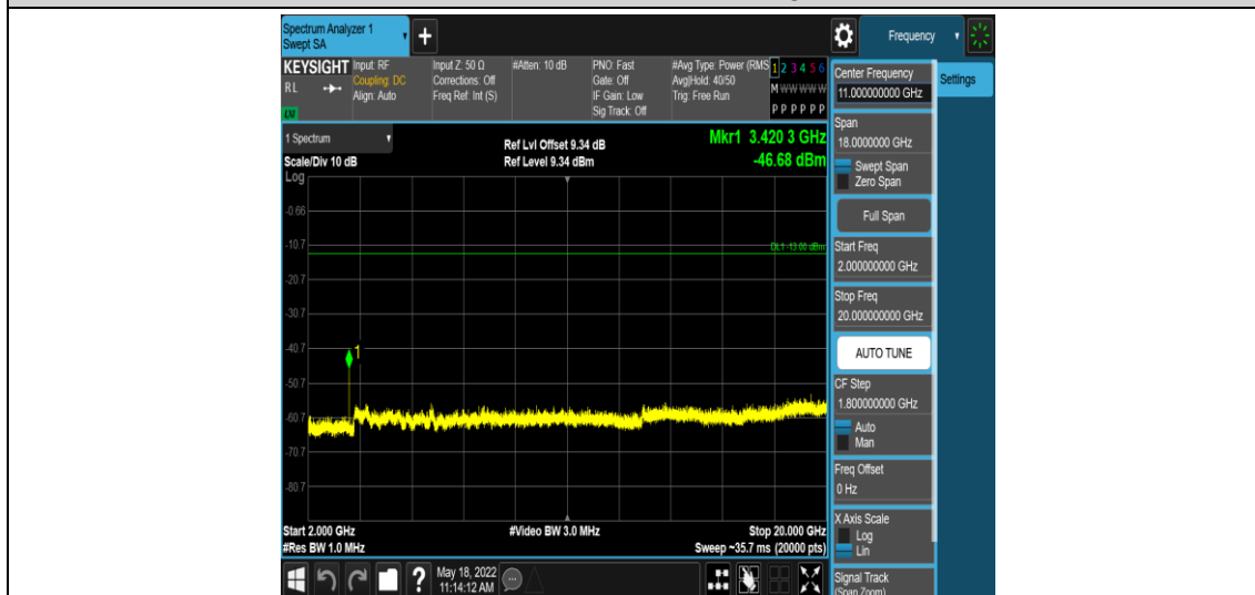
Band4-1.4MHz-16QAM-19957-1RB#0-Range5:2000~20000MHz
