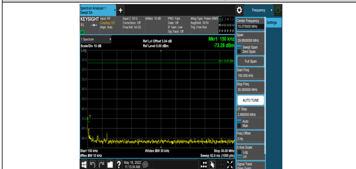
Band4-1.4MHz-16QAM-19957-1RB#0-Range2:0.15~30MHz
